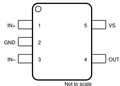
Figure 6-1. INA180-Q1: DBV Package 5-Pin SOT-23 (Pinout A) Top View Figure 6-2. INA180-Q1: DBV Package 5-Pin SOT-23 (Pinout B) Top View
