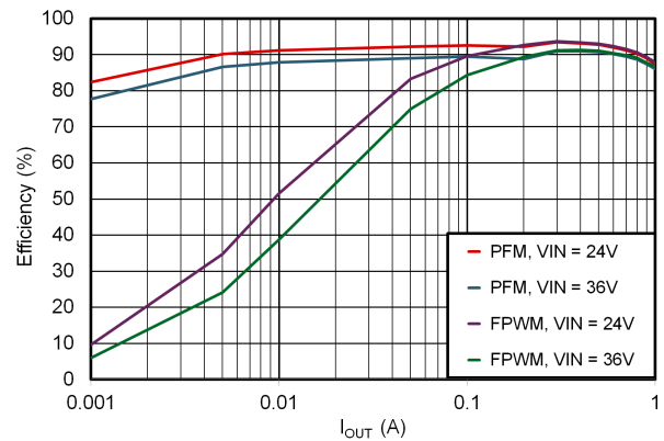
Figure 6-4. 3.3V Efficiency Versus Load Current
