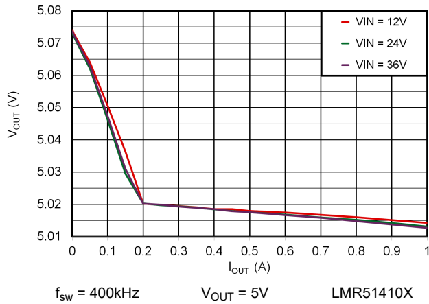
Figure 6-7. 5V load Regulation
