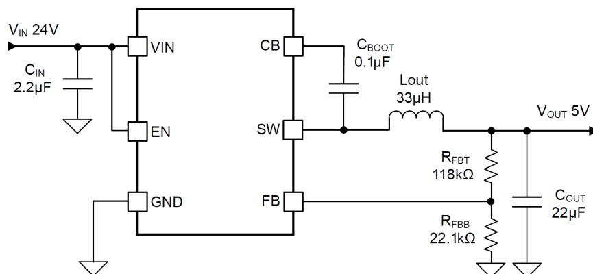
Figure 8-1. Application Circuit
