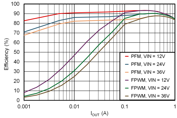
Figure 6-2. 5V Efficiency Versus Load Current
