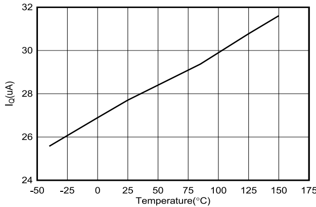
Figure 6-9. V_{IN} Quiescent Current Versus Temperature
