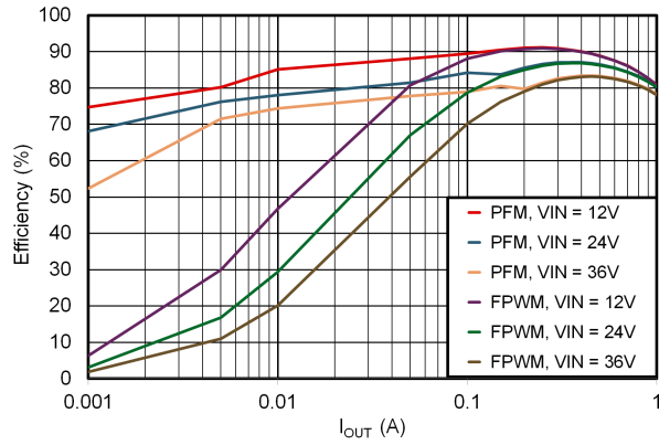
Figure 6-1. 3.3V Efficiency Versus Load Current
