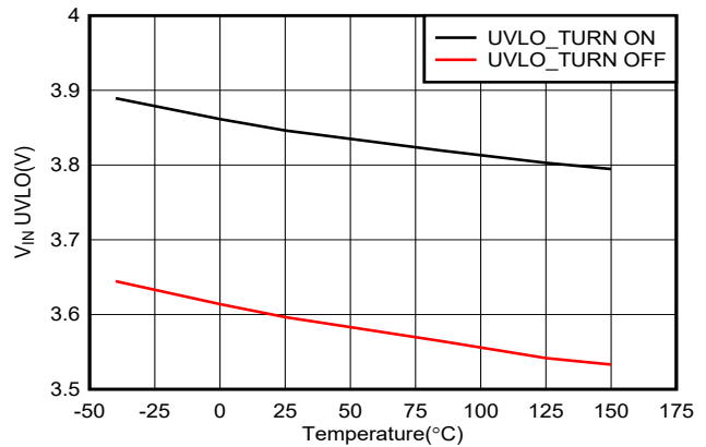
Figure 6-10. V_{IN} UVLO Versus Temperature
