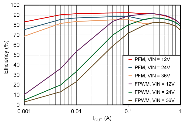
Figure 6-3. 12V Efficiency Versus Load Current
