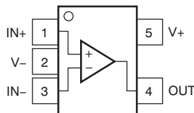
OPA171 DRL Package 5-Pin SOT-553 Top View
