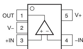
OPA171 DBV Package 5-Pin SOT-23 Top View
