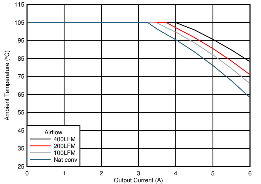
Figure 3. LMZM33606 SOA Curve for 24-V Input and 5-V Output
