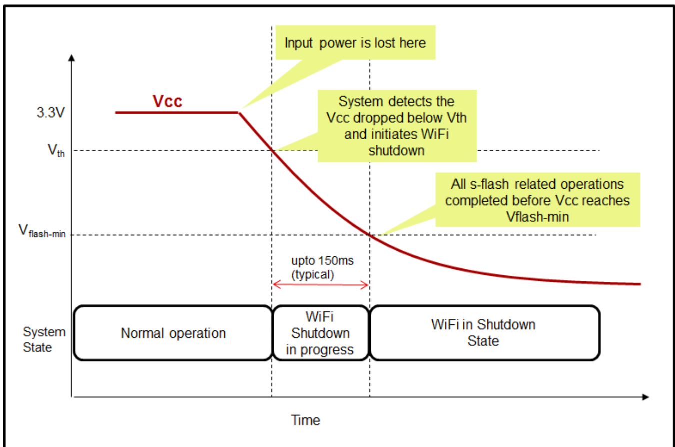
Figure 2. Sudden Power Off in Line-Powered Device
