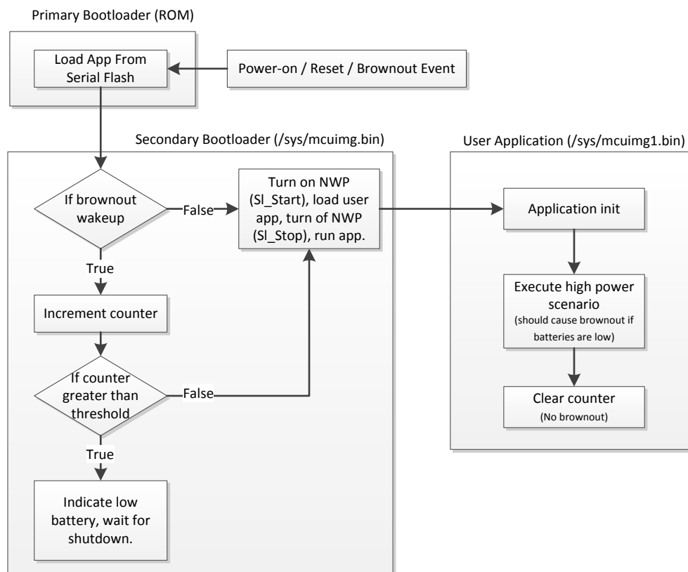
Figure 3. Brownout Suggested Flow
