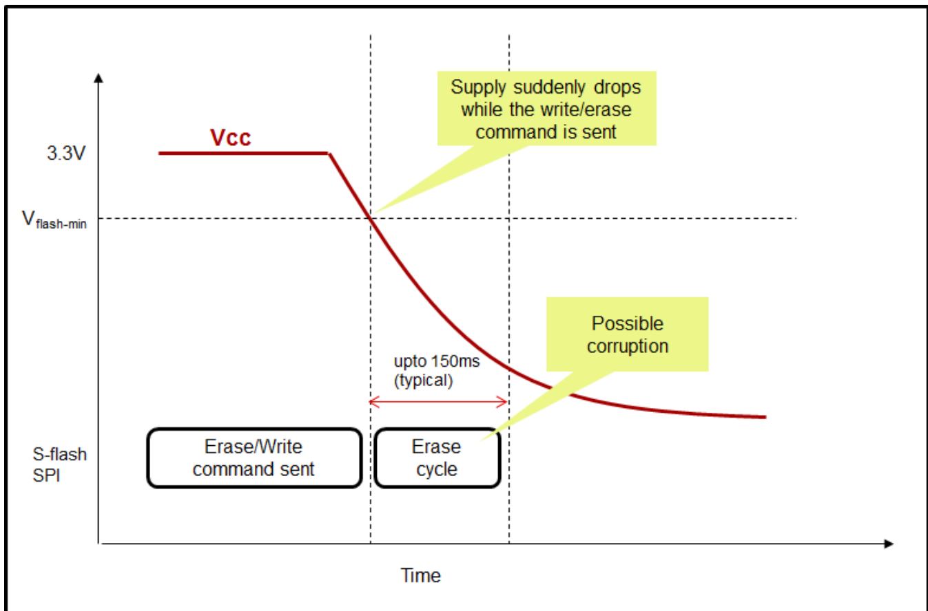
Figure 1. Sudden Power Off During Flash Erase
