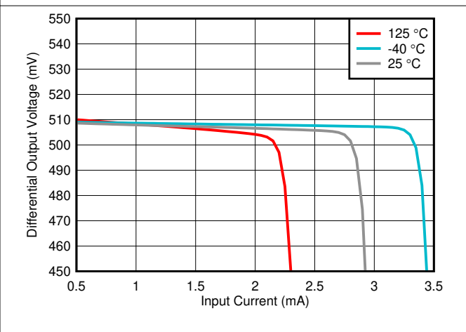
图 6-42. Ambient Light Cancellation Range vs Ambient Temperature
