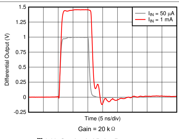
图 6-22. Overloaded Pulse Response
