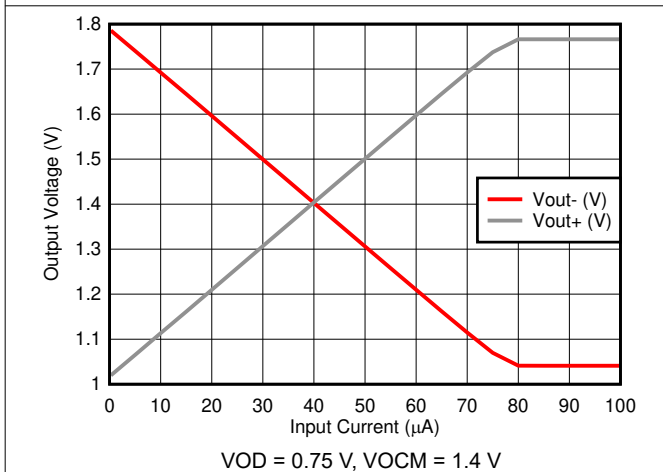
图 6-39. High-side Swing vs Input Current
