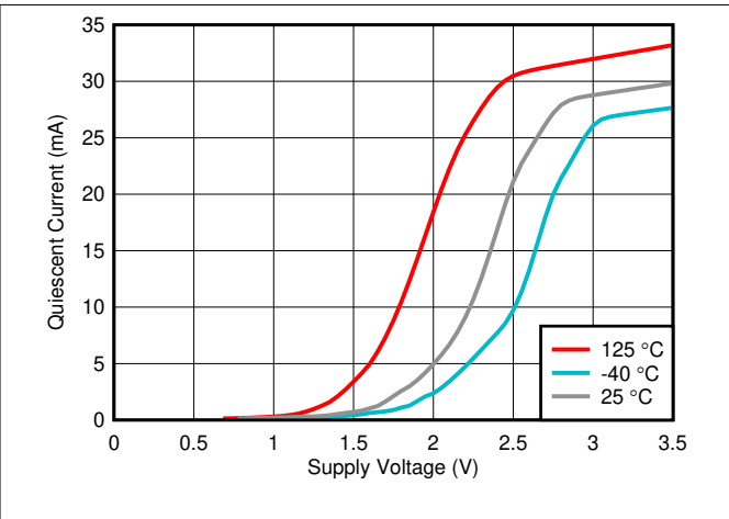
图 6-38. Quiescent Current vs Supply Voltage
