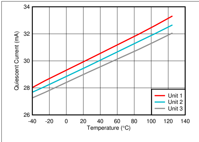
图 6-37. Quiescent Current vs Ambient Temperature
