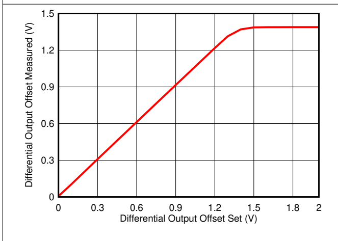
图 6-41. Differential Output Offset Gain
