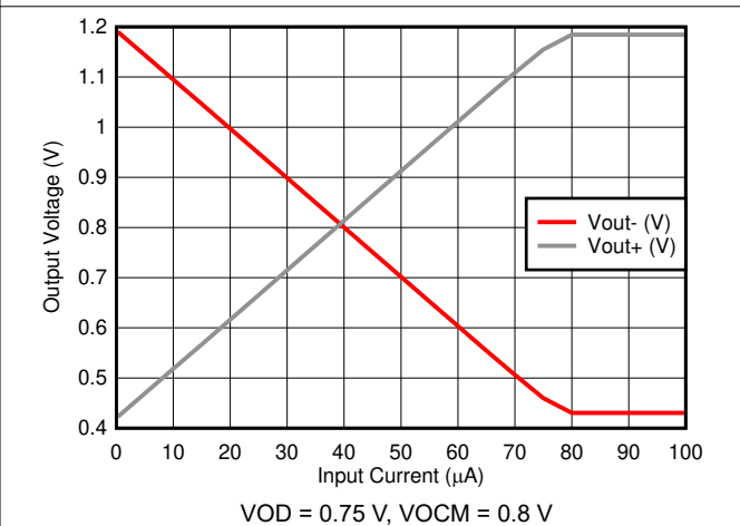
图 6-40. Low-side Swing vs Input Current
