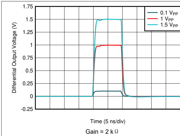
图 6-19. Pulse Response vs Output Swing
