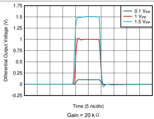
图 6-20. Pulse Response vs Output Swing
