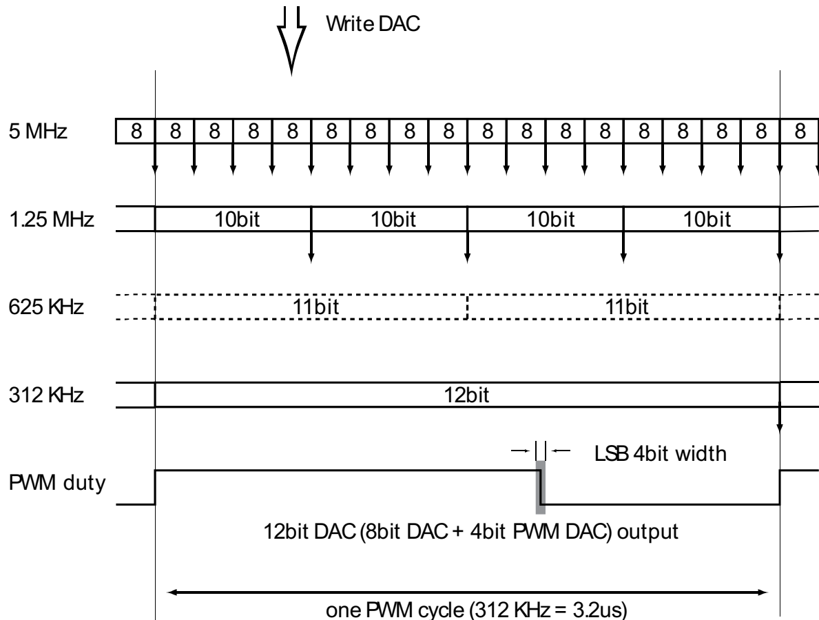
Figure 49. Example of 12-Bit DAC Conversion Time (FCS/TRK/TLT)
