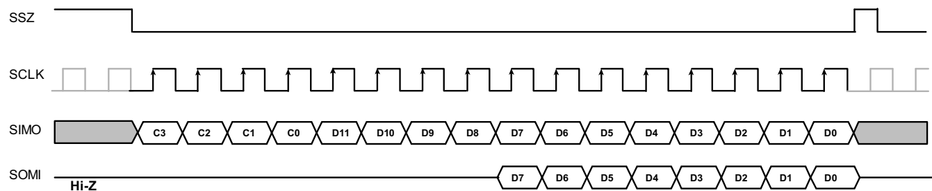
Figure 12. Write 12 Bits Focus DAC Data + Read 8 Bits Status Data
