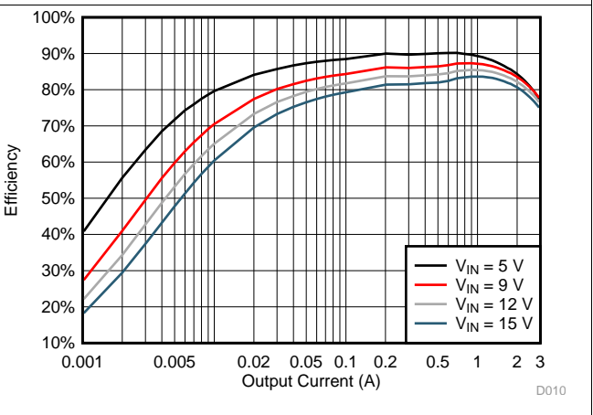
Figure 10. TPS563201 V_{OUT} = 1.5\text{ V} Efficiency, L = 2.2\ \mu\text{H}
