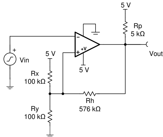
图 8-1. Comparator Schematic With Hysteresis
