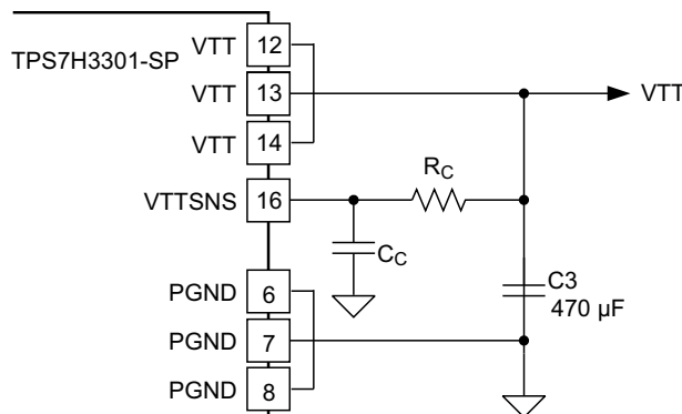
Figure 22. R-C Filter for VTTSNS
