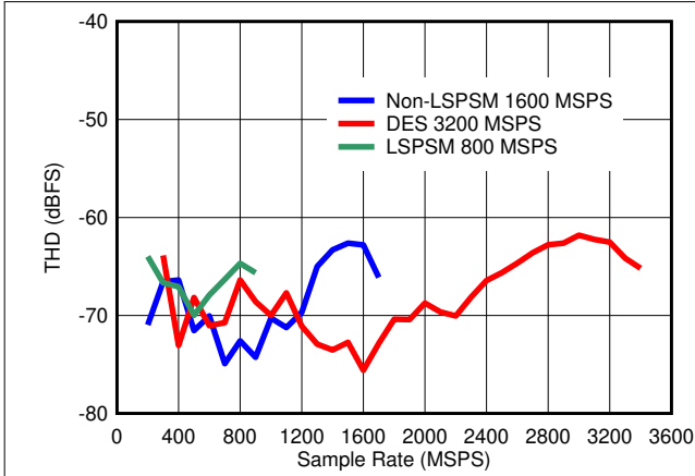
图 6-23. THD vs Sample Rate
