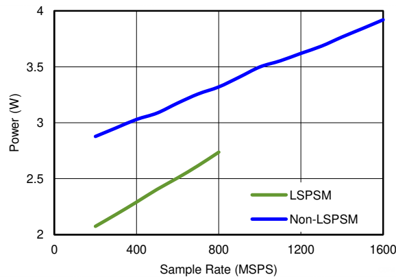
图 6-39. Power Consumption vs Sample Rate
