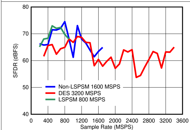
图 6-27. SFDR vs Sample Rate
