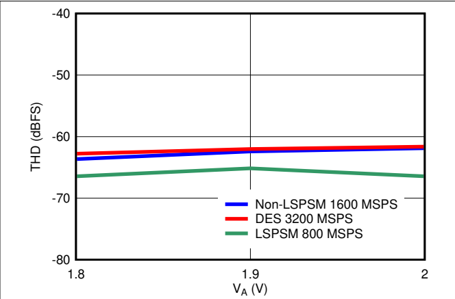
图 6-24. THD vs Supply Voltage
