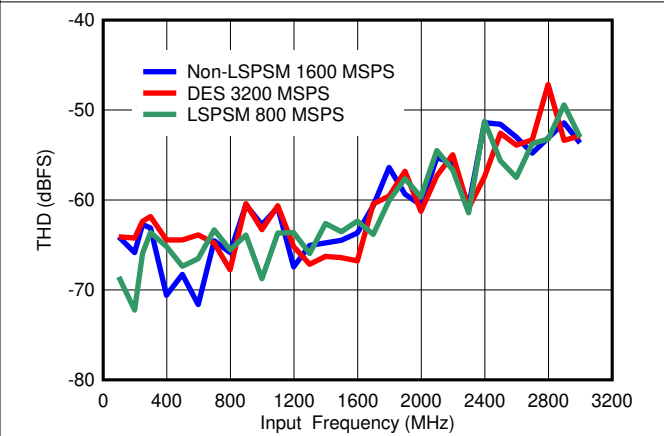
图 6-26. THD vs Input Frequency
