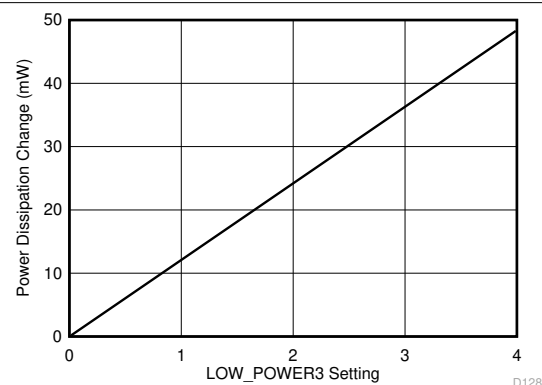
图 6-11. Power Dissipation Change vs LOW_POWER3 register setting
