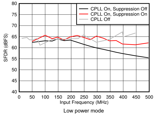
图 5-44. SFDR vs F_{IN} and C-PLL modes
