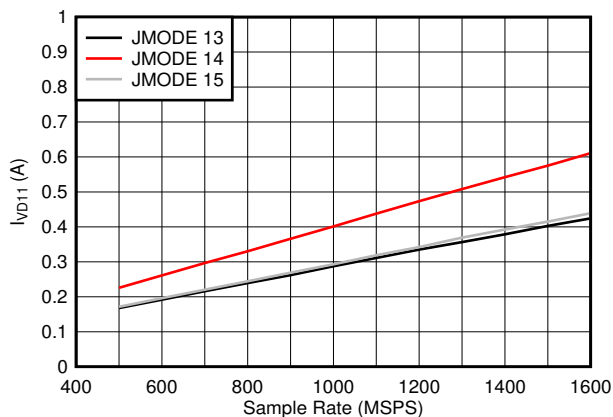
图 5-88. Quad Channel, I_{D11} vs F_S and JMODE 13 - 15
