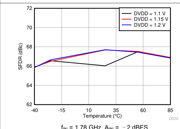
图 6-48. Spurious-Free Dynamic Range vs. DVDD Supply and Temperature
