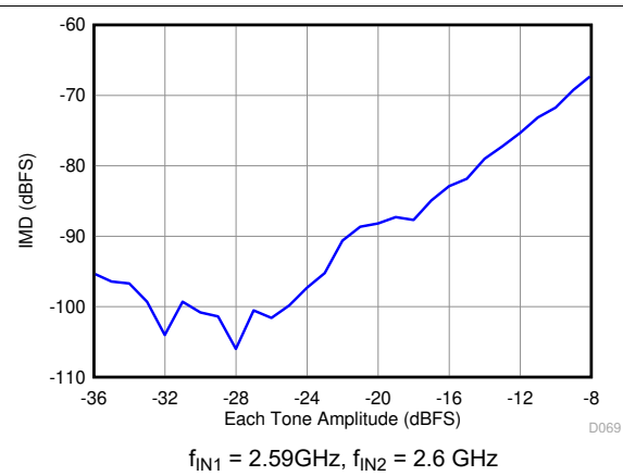
图 6-36. Intermodulation Distortion vs. Input Amplitude (3490 MHz and 3510 MHz, f_s = 2457.6 MSPS)
