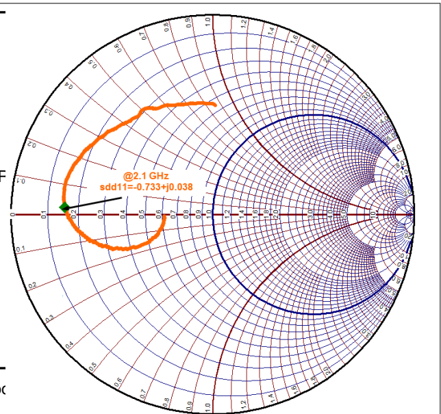
图 8-2. SDD11 Over the Input Frequency Range
