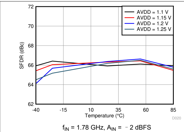
图 6-44. Spurious-Free Dynamic Range vs. AVDD Supply and Temperature
