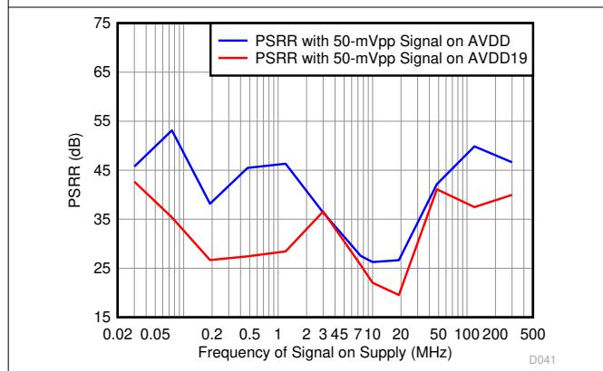
图 6-65. Power-Supply Rejection Ratio vs. Tone Frequency
