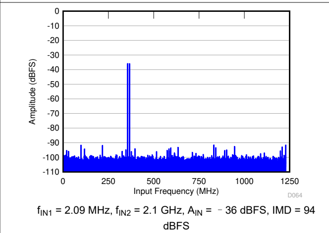
图 6-26. FFT for Two-Tone Input Signal (-36 dBFS, f_s = 2457.6 \text{ MSPS} )
