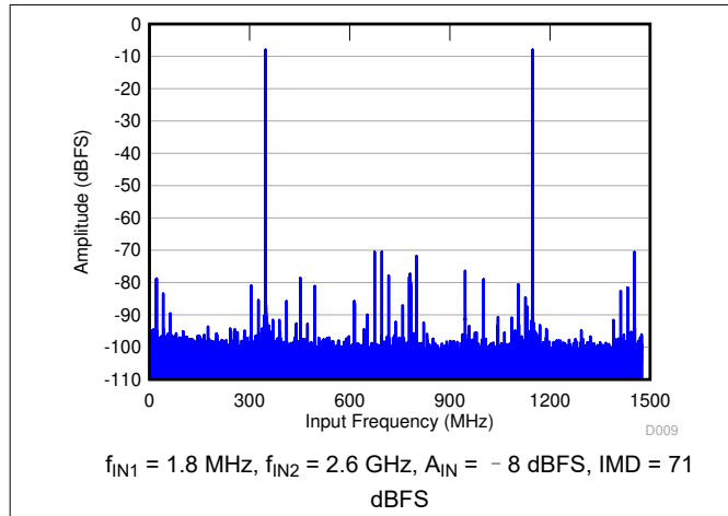
图 6-23. FFT for Two-Tone Input Signal (-8 dBFS)
