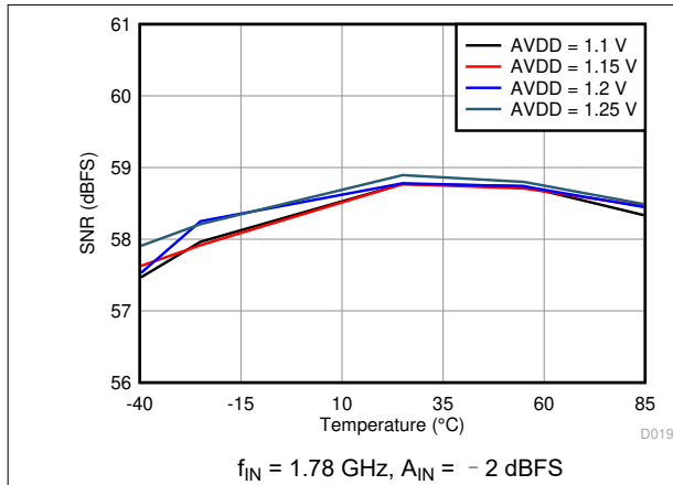
图 6-43. Signal-to-Noise Ratio vs. AVDD Supply and Temperature
