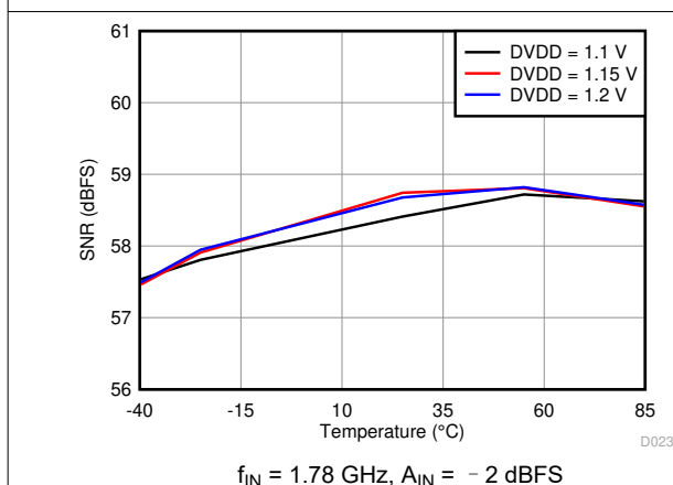
图 6-47. Signal-to-Noise Ratio vs. DVDD Supply and Temperature
