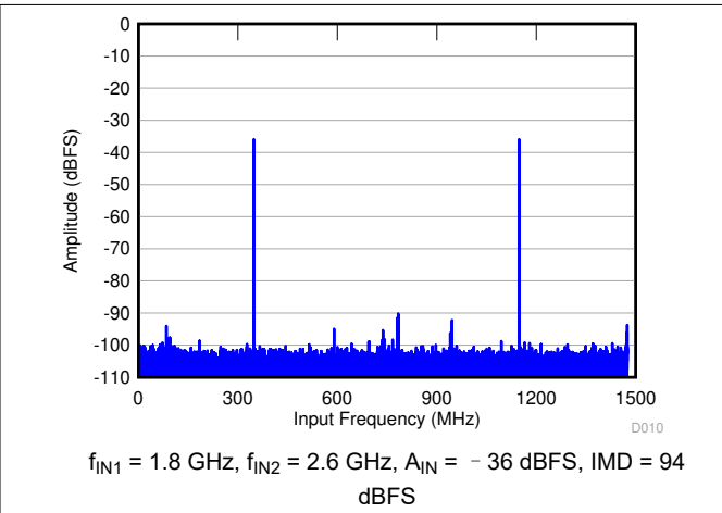
图 6-24. FFT for Two-Tone Input Signal
