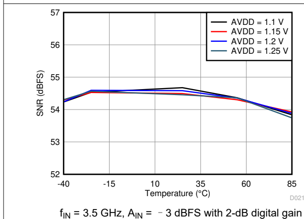
图 6-45. Signal-to-Noise Ratio vs. AVDD Supply and Temperature
