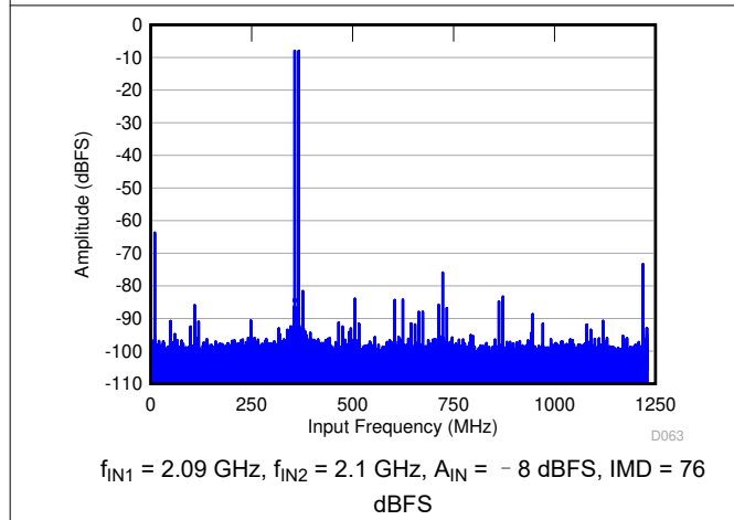
图 6-25. FFT for Two-Tone Input Signal (-8 dBFS, f_s = 2457.6 \text{ MSPS} )
