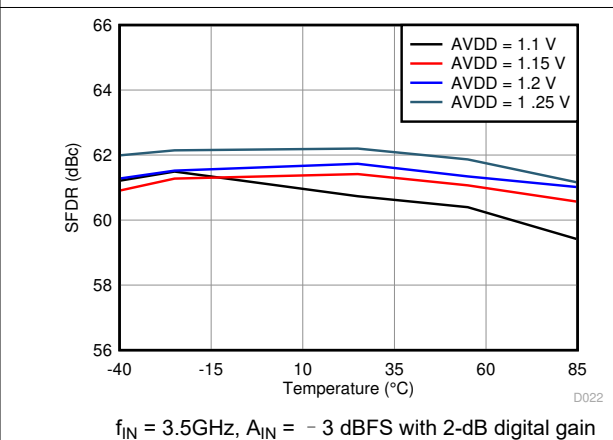
图 6-46. Spurious-Free Dynamic Range vs. AVDD Supply and Temperature
