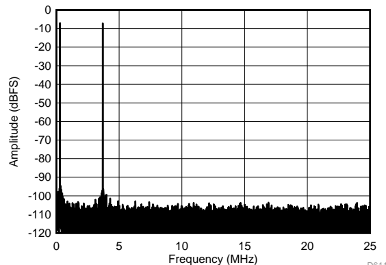
f_{IN1} = 46\text{ MHz} , f_{IN2} = 50\text{ MHz} , IMD3 = 102 dBFS, each tone at -7\text{ dBFS}
