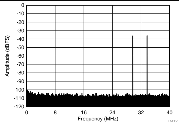
f_{IN1} = 46\text{ MHz} , f_{IN2} = 50\text{ MHz} , IMD3 = 105 dBFS, each tone at -36\text{ dBFS}
