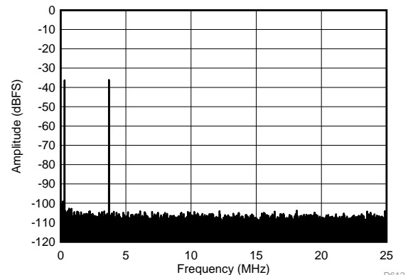
f_{IN1} = 46.3\text{ MHz} , f_{IN2} = 50.3\text{ MHz} , IMD3 = 110 dBFS, each tone at -36\text{ dBFS}
