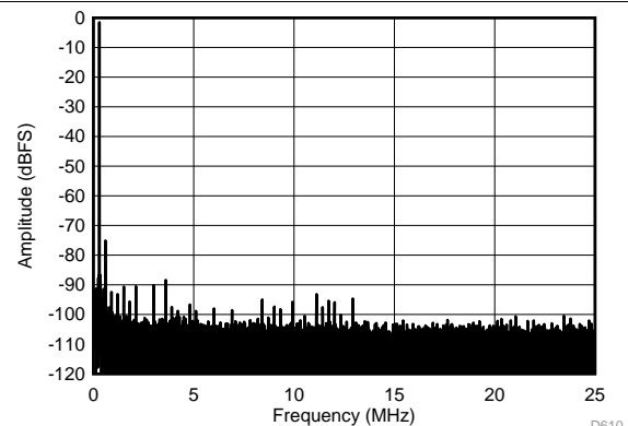
SFDR = 68 dBc, SNR = 67.5 dBFS, SINAD = 67.4 dBFS, THD = -87\text{ dBc} , HD2 = -68\text{ dBc} , HD3 = -87\text{ dBc}
