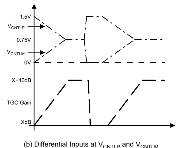
Figure 84. V_{\text{CNTLP}} and V_{\text{CNTLM}} Configurations
