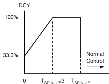
图 8-14. Spin-Up Process
