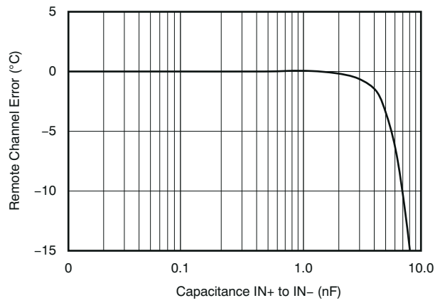
图 7-9. Temperature Error vs Capacitance Between IN+ and IN-
