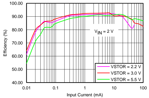
V_{IN\_DC} = sourcemeter configured with voltage source = 2.0 V and I_{COMP} varied from 0.01 mA to 100 mA VSTOR = sourcemeter configured to measure current and voltage source set to hold the VSTOR voltage = 2.2 V, 3.0 V or 5.5 V
