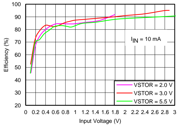
V_{IN\_DC} = sourcemeter configured with I_{COMP} = 10 mA and voltage source varied from 0.1 V to 3.0 V VSTOR = sourcemeter configured to measure current and voltage source set to hold the VSTOR voltage = 2.0 V, 3.0 V or 5.5 V
