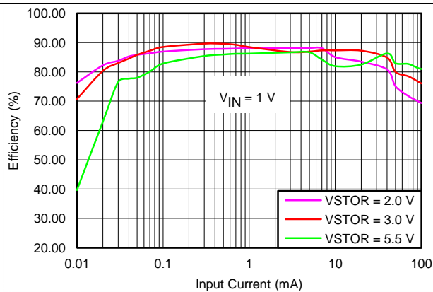
V_{IN\_DC} = sourcemeter configured with voltage source = 1.0 V and I_{COMP} varied from 0.01 mA to 100 mA VSTOR = sourcemeter configured to measure current and voltage source set to hold the VSTOR voltage = 2.0 V, 3.0 V or 5.5 V
