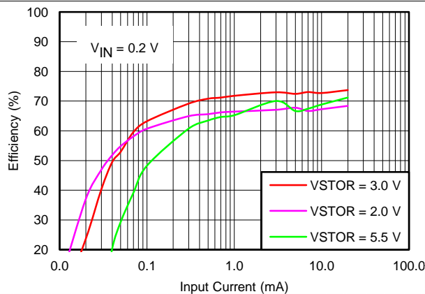
V_{IN\_DC} = sourcemeter configured with voltage source = 0.2 V and I_{COMP} varied from 0.01 mA to 100 mA VSTOR = sourcemeter configured to measure current and voltage source set to hold the VSTOR voltage = 2.0 V, 3.0 V or 5.5 V
