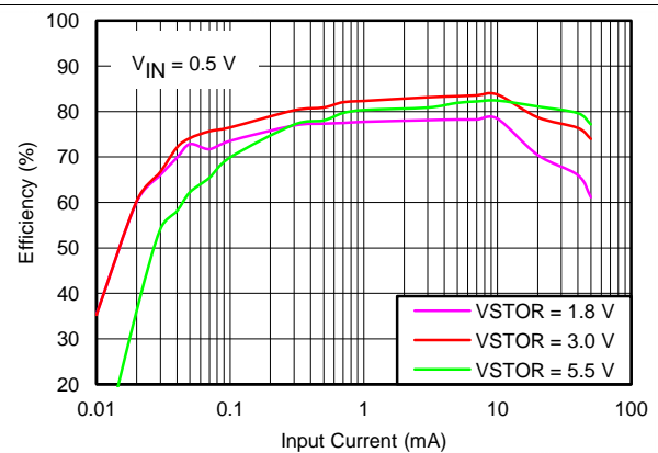
V_{IN\_DC} = sourcemeter configured with voltage source = 0.5 V and I_{COMP} varied from 0.01 mA to 100 mA VSTOR = sourcemeter configured to measure current and voltage source set to hold the VSTOR voltage = 1.8 V, 3.0 V or 5.5 V
