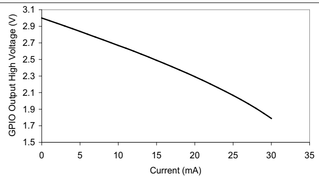
Figure 4-10. GPIO Output High Voltage vs Current Being Sourced
