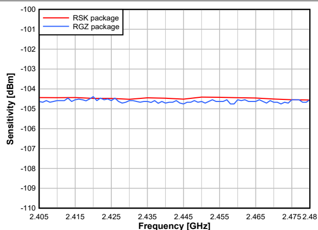
图 7-11. Sensitivity vs. Frequency (IEEE 802.15.4 OQPSK DSSS1:8, 250kbps, 2.44GHz)
