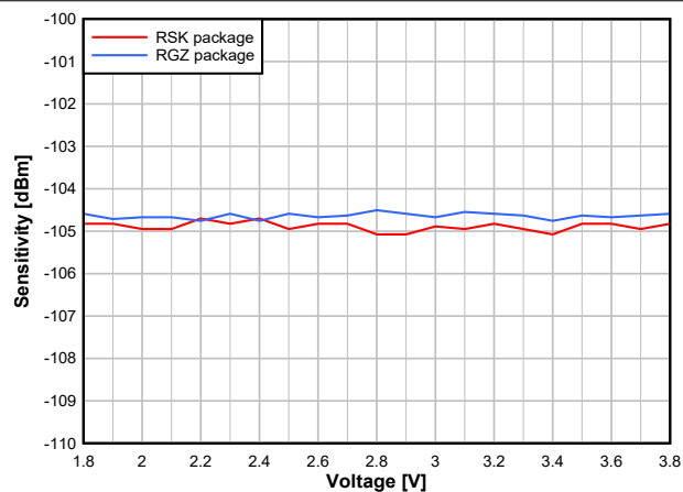
图 7-15. Sensitivity vs. Supply Voltage (VDD) (250kbps, 2.44GHz)
