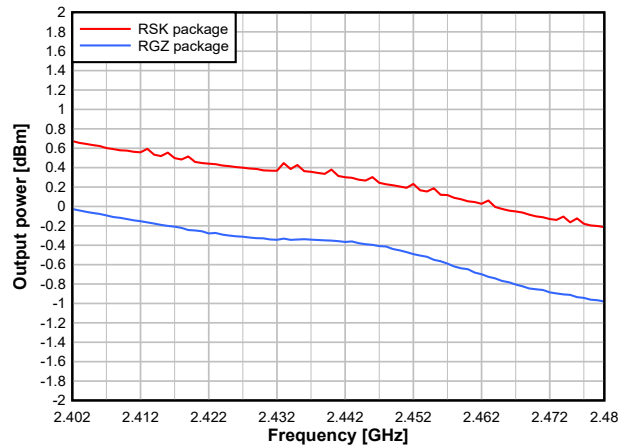
图 7-20. Output Power vs. Frequency (BLE 1Mbps, 2.44GHz, 0dBm)
