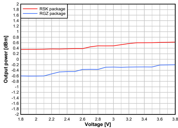
图 7-18. Output Power vs. Supply Voltage (VDD5) (BLE 1Mbps, 2.44GHz, 0dBm)
