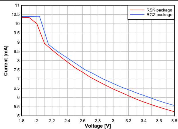
图 7-7. RX Current vs. Supply Voltage (VDD) (BLE 1Mbps, 2.44GHz)
