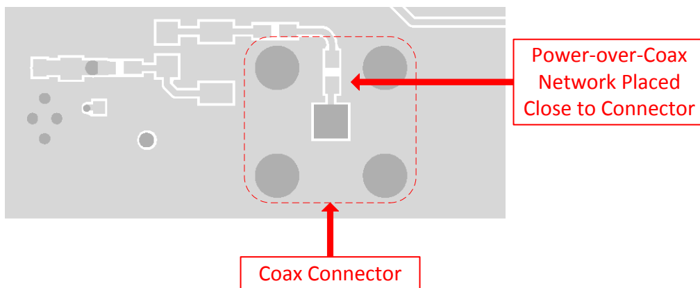
图 10-2. Power-over-Coax Layout
