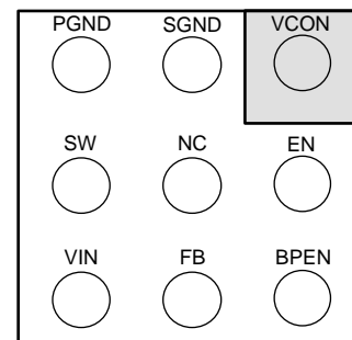
YFQ Package 9-Pin DSBGA Bottom View
