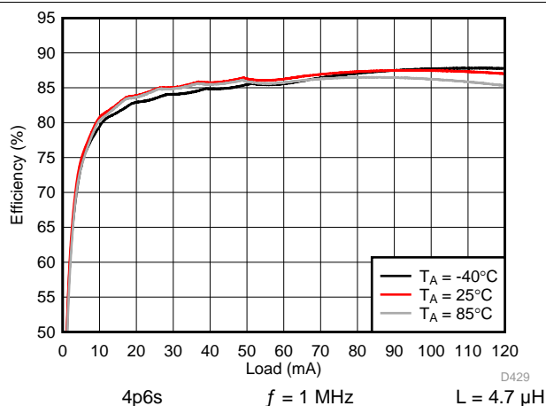
图 177. Backlight Boost Efficiency
