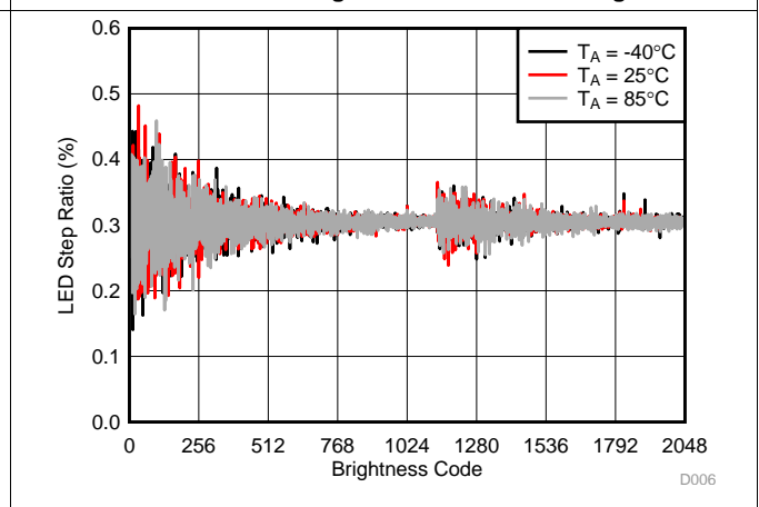
图 7. Backlight LED Current-Step Ratio
