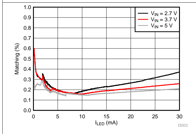
图 4. Backlight LED Current Matching
