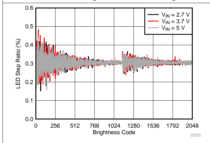
图 6. Backlight LED Current-Step Ratio
