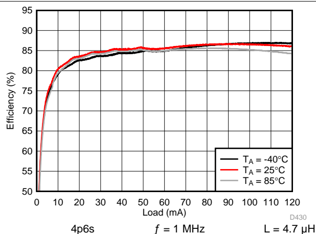
图 178. Backlight System Efficiency
