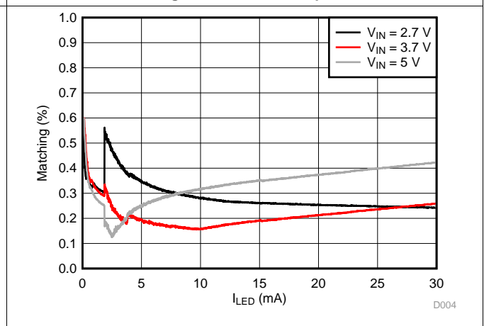
图 5. Backlight LED Current Matching
