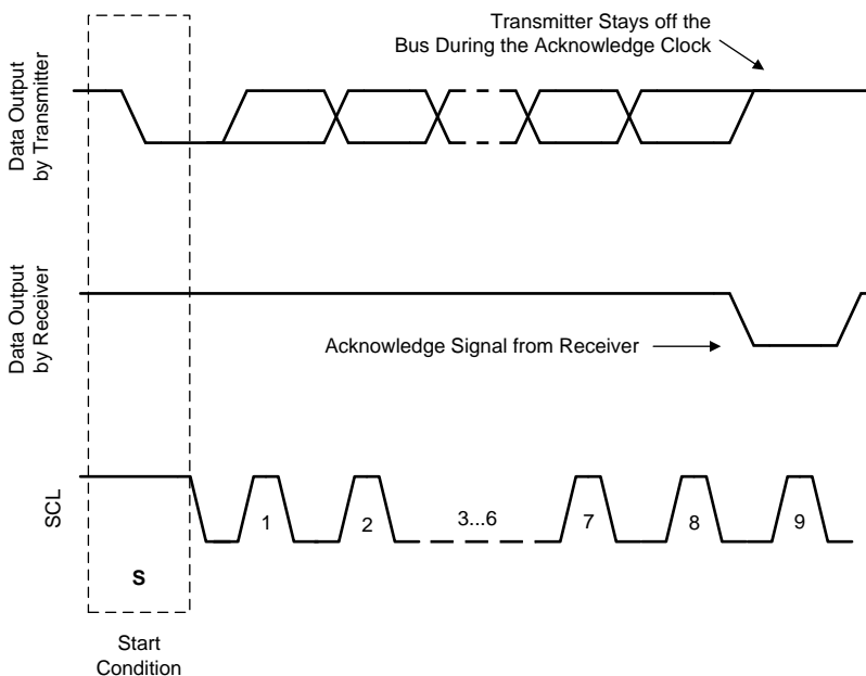
图 43. Acknowledge Signal
