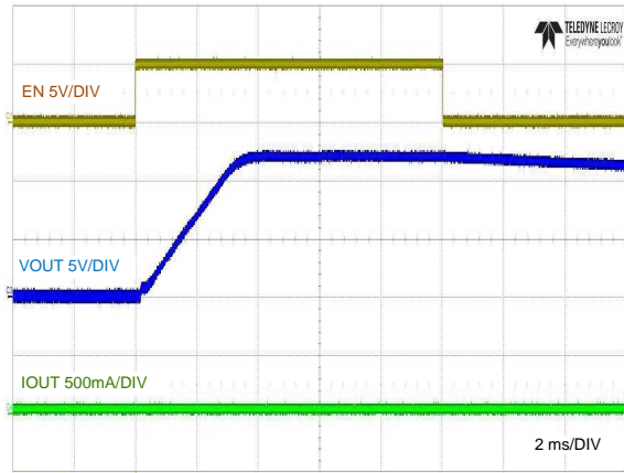
图 19. No-Load Start-up and Shutdown with EN/UVLO
