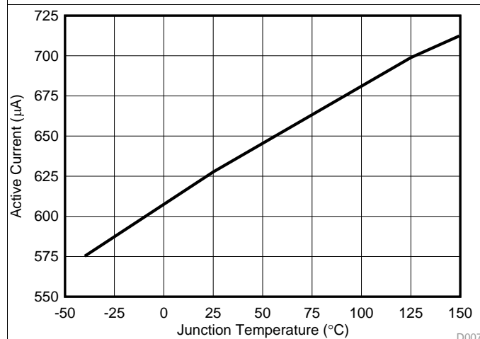
图 5. V_{IN} Active Current vs. Temperature
