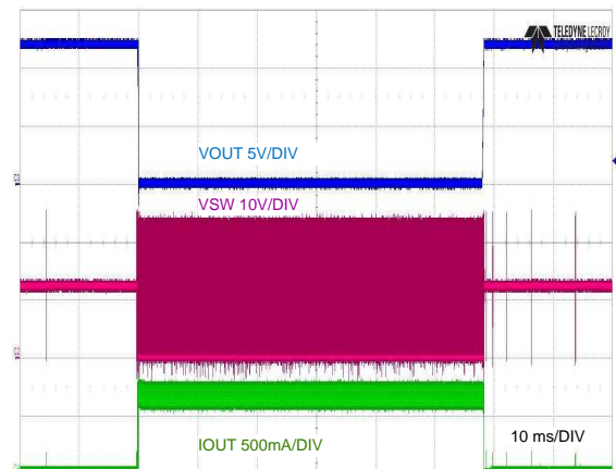
图 22. Short Circuit Applied
