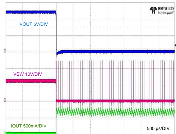
图 20. Full-Load Start-up and Shutdown with EN/UVLO
