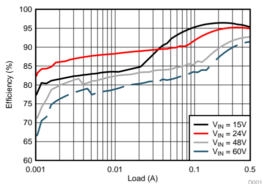
典型应用效率, V_{OUT} = 12\text{V}
