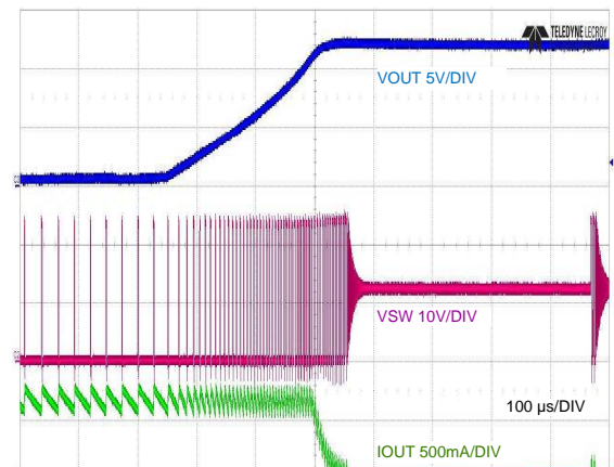
图 21. Pre-bias Start-up with EN/UVLO
