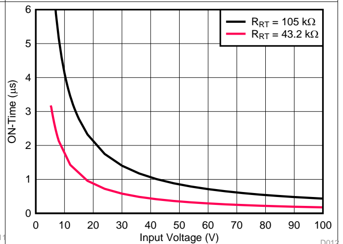
图 10. COT On-Time vs. V_{IN}
