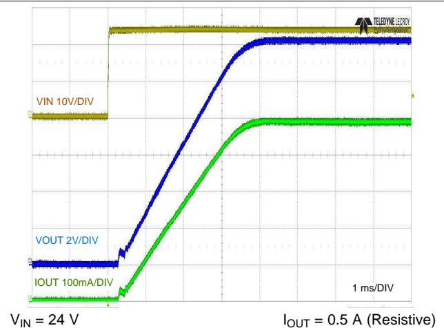
图 18. Full-Load Start-up with V_{IN}
