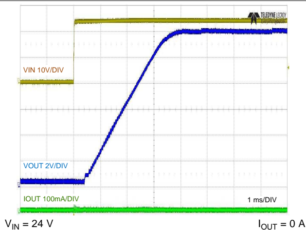
图 17. No-Load Start-up with V_{IN}
