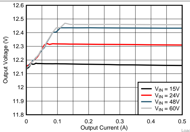
图 15. Load and Line Regulation Performance
