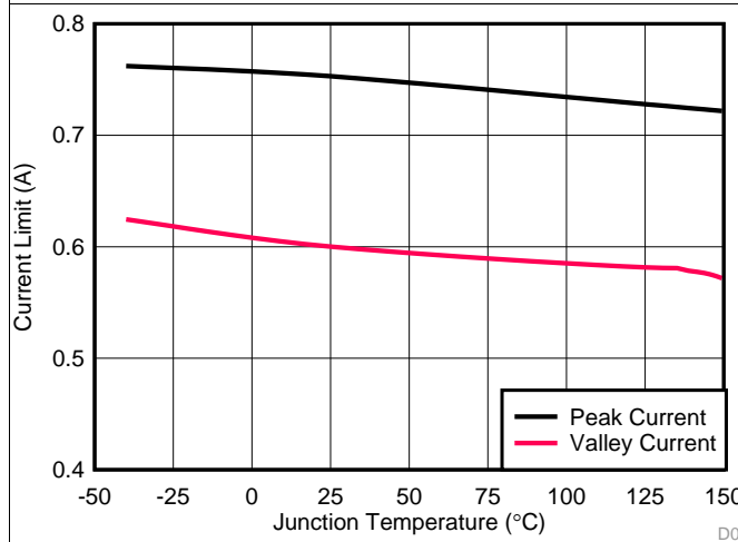
图 9. Peak and Valley Current Limit vs. Temperature
