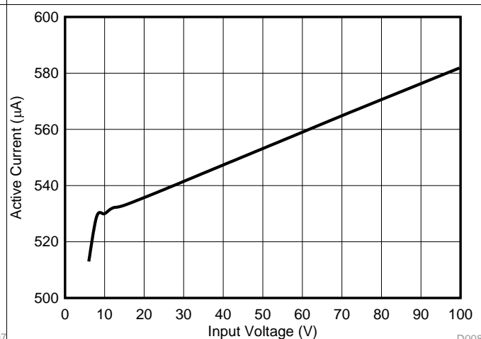
图 6. V_{IN} Active Current vs. Input Voltage
