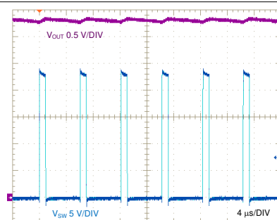
V_{IN} = 24\text{ V} I_{OUT} = 150\text{ mA} 图 8-28. SW Node and Output Ripple Voltages, Full Load
