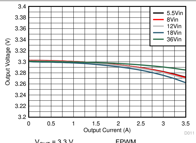
图 9-22. Load and Line Regulation
