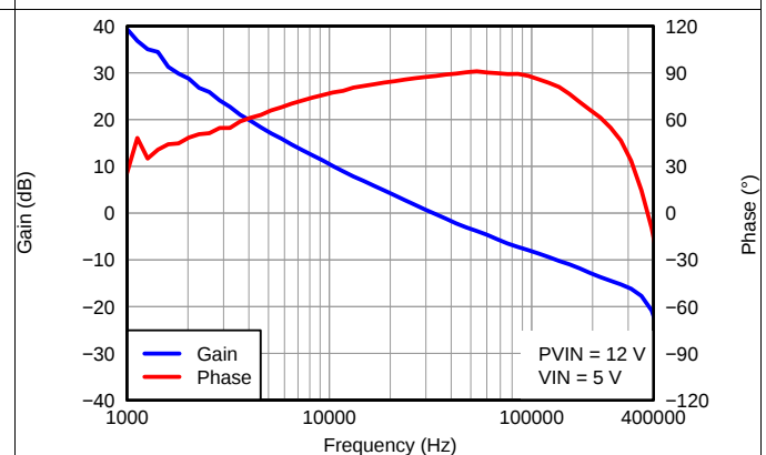
图 16. V OUT =1.2 V, I OUT =3 A, C OUT1 =47 µF ceramic, C OUT2 = 330 µF POSCAP, f SW =480 kHz, P VIN = 12 V, V IN = 5 V
