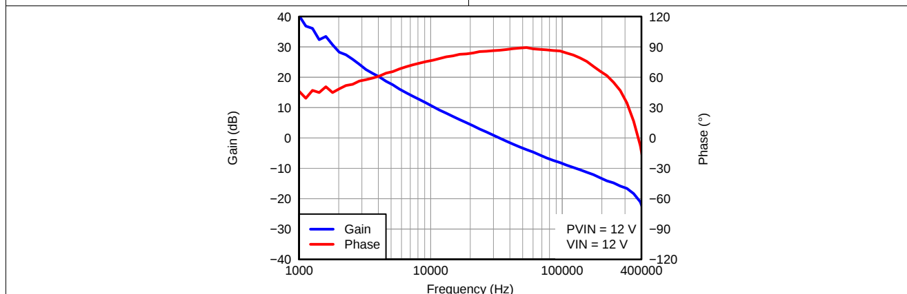
图 5. VOUT=1.2 V, IOUT=3 A, COUT1=47 μF ceramic, COUT2= 330 μF POSCAP, fSW=480 kHz
