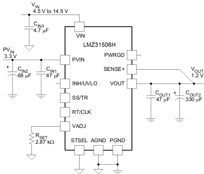
图 27. Typical Schematic PVIN = 3.3 V, VIN = 4.5 V to 14.5 V, VOUT = 1.2 V
