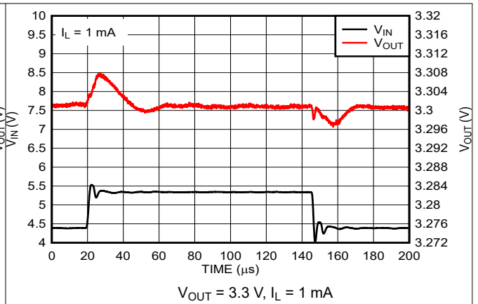
图 7-8. Line Transient Response (New Chip)
