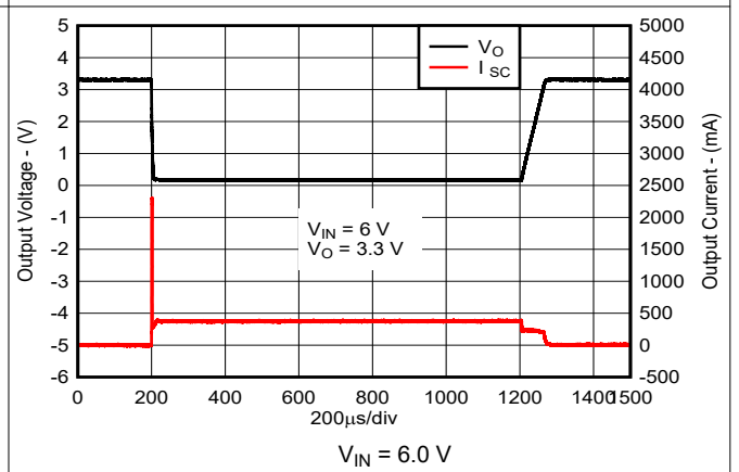
图 5-16. Short Circuit Current vs Time (New Chip)
