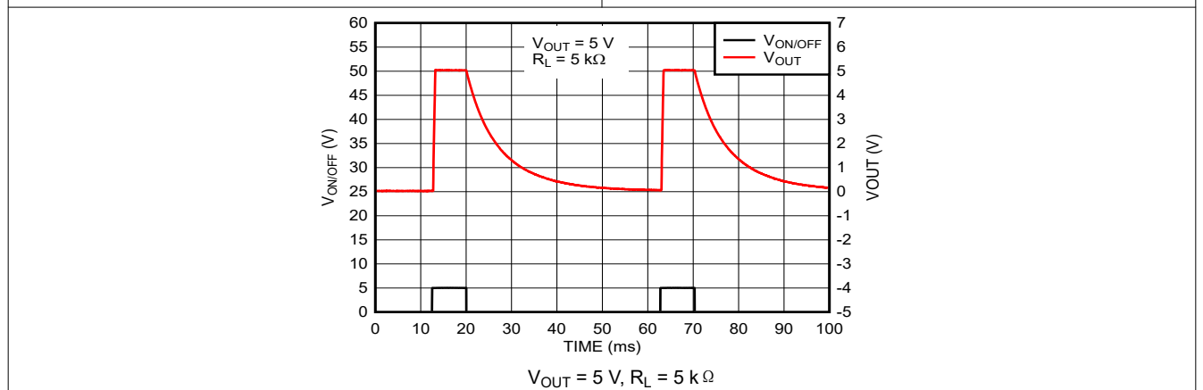
图 7-11. Turn-off Waveform (New Chip)
