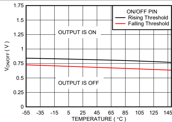
图 5-29. ON/ OFF Threshold vs Temperature (New Chip)
