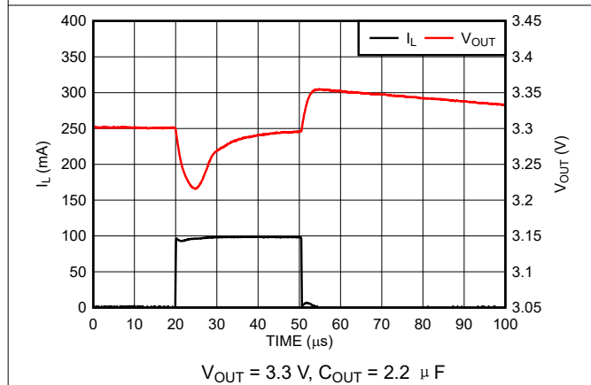
图 7-9. Load Transient Response (New Chip)
