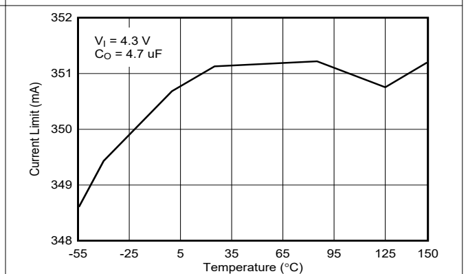
图 5-18. Instantaneous Short Circuit Current vs Temperature (New Chip)
