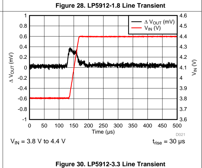
Figure 28. LP5912-1.8 Line Transient
