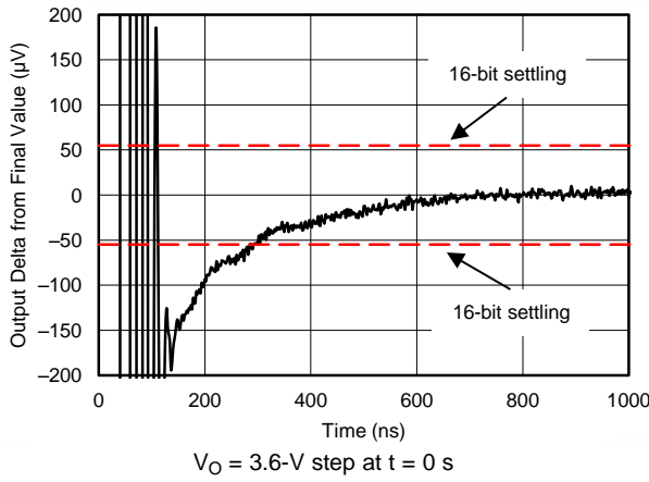
图 32. 16-Bit Negative Settling Time
