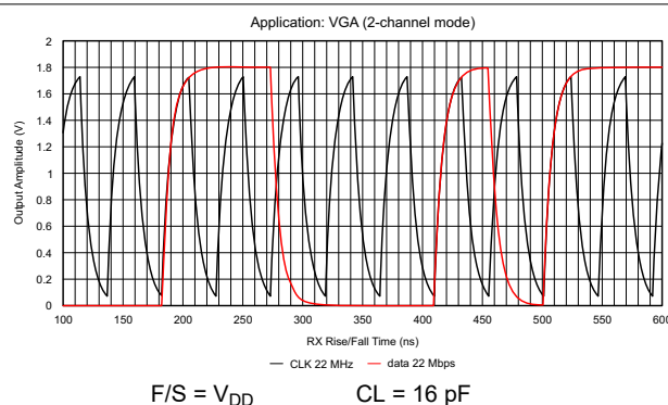
图 9-3. Output Amplitude vs Toggling Frequency (F/S = 1)
