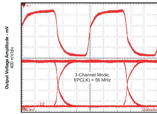
图 6-13. XGA 3-Channel Output Waveform
