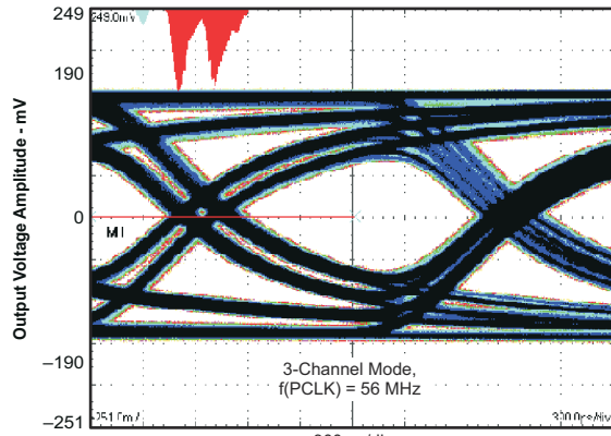
图 6-12. XGA 3-Channel Output Waveform
