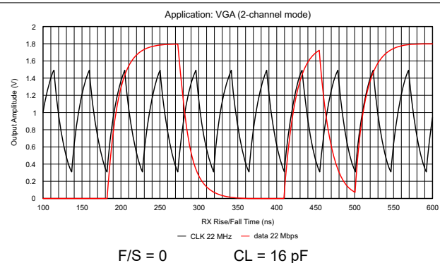
图 9-4. Output Amplitude vs Toggling Frequency (F/S = 0)
