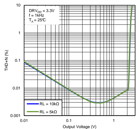
Figure 36. Line Driver THD+N vs Output Voltage
