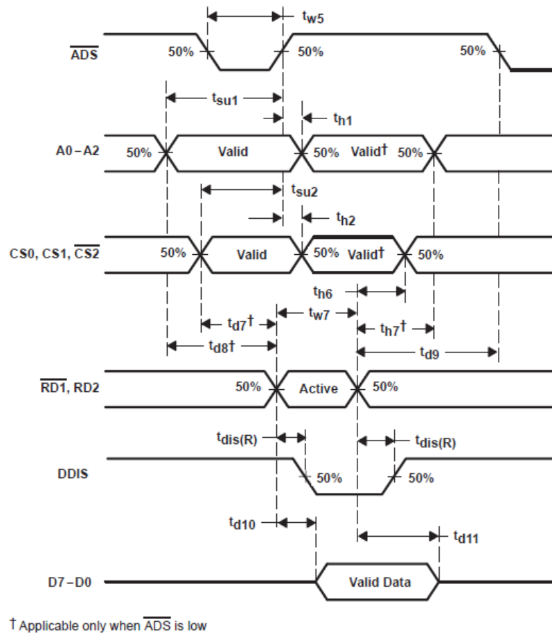
图 6-3. Read Cycle Timing Waveforms
