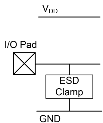
图 23-16. ESD Protection on Fail-Safe Pins
