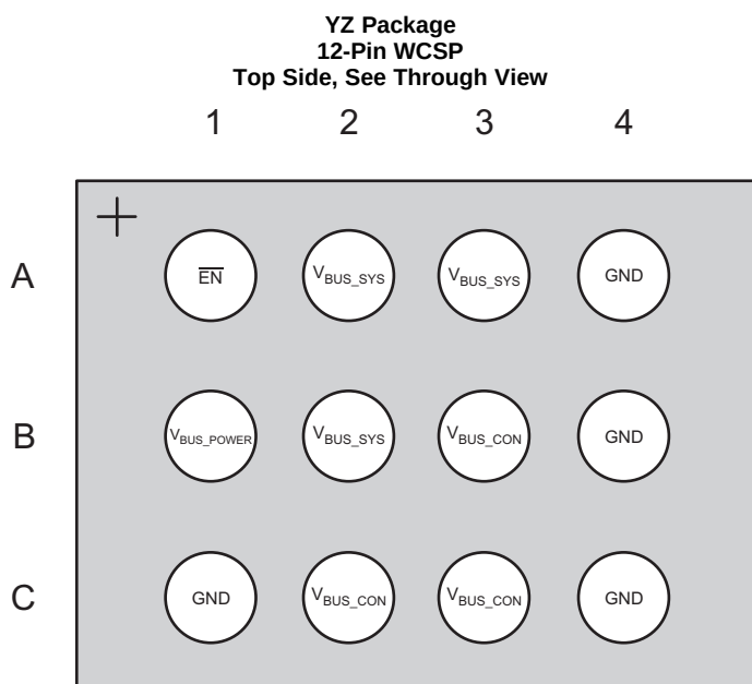
Pin Functions
