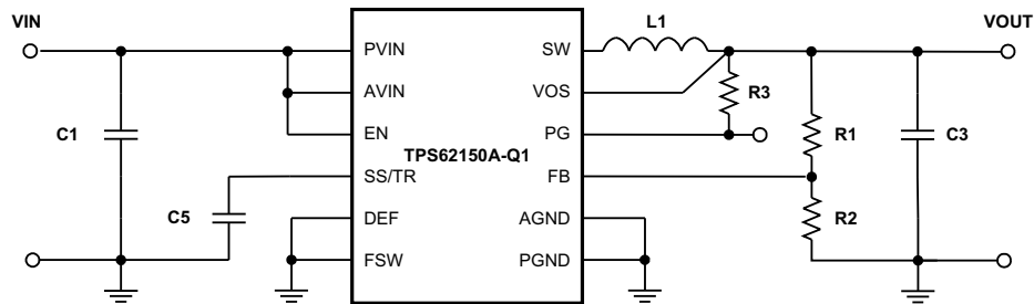
Figure 5. Measurement Setup (High Switching Frequency)
