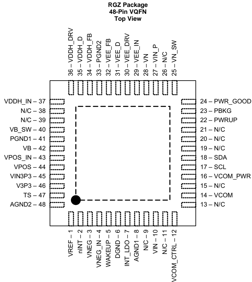
Pin Functions
