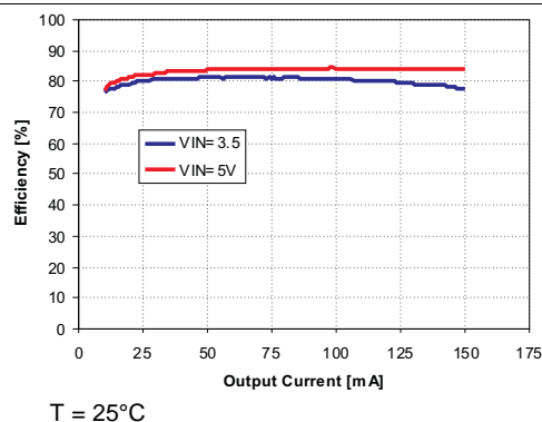
Figure 30. VB DCDC Efficiency
