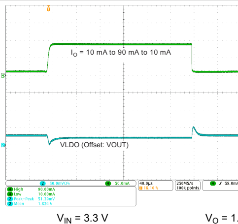
图 9-17. LDO6, LDO8 Load Transient Response
