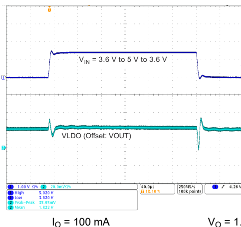
图 9-19. LDO6, LDO8 Line Transient Response
