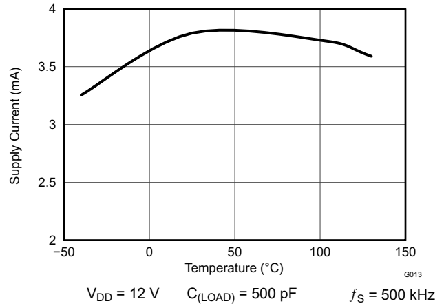
图 5-6. Operating Supply Current vs Temperature (Output Switching)
