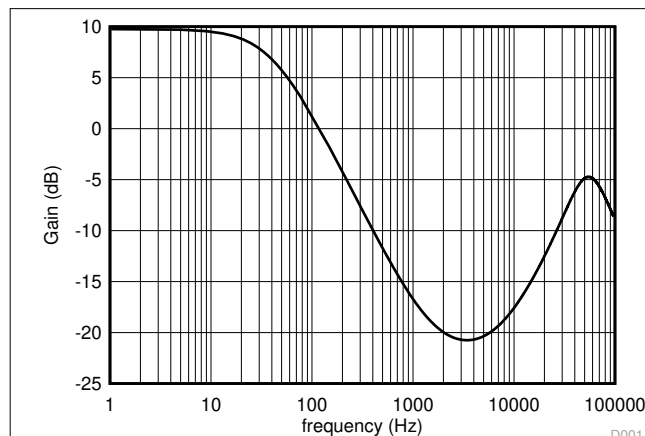
图 9-4. Converter Open-Loop Bode Plot - Gain
