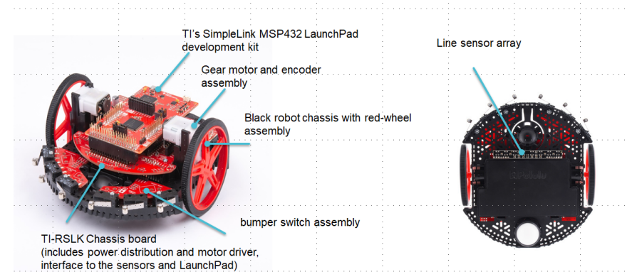
Fully assembled TI-RSLK MAX robot
