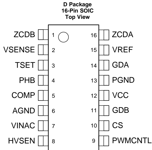
Pin Functions
