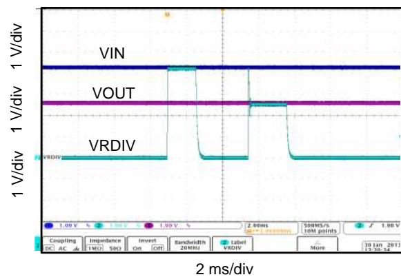
Figure 34. Sampling Waveform
