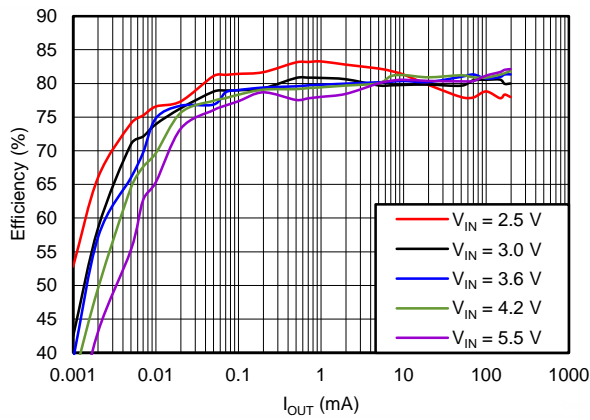
Figure 44. Efficiency Vs Output Current, V_{OUT} = 1.3\text{ V}
