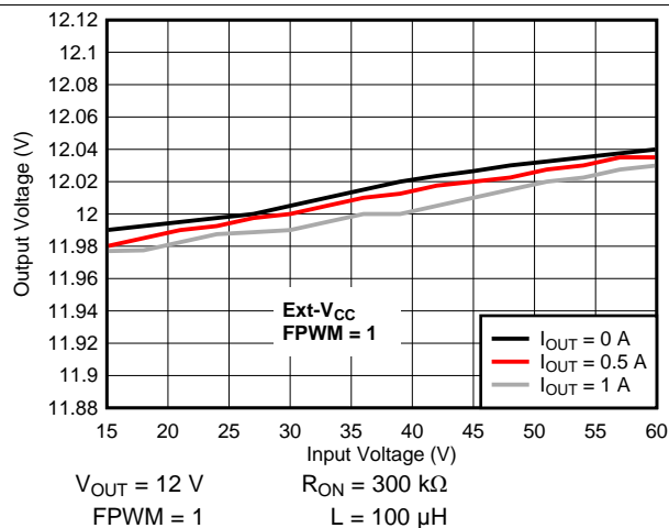
图 5. Line Regulation
