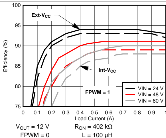
图 3. Efficiency at 300 kHz
