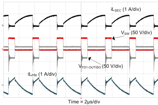
图 37. Steady State at V_{IN} = 48\text{ V} and I_{OUT2} = 500\text{ mA}
