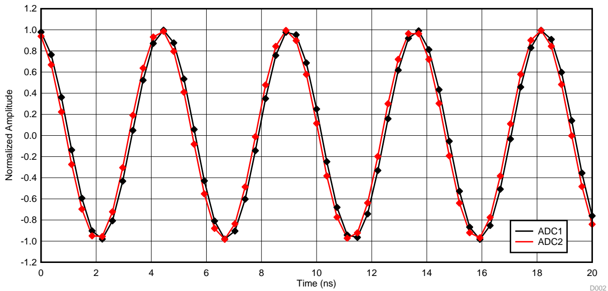
图 18. Sampled Signals at 2482-MHz Input
