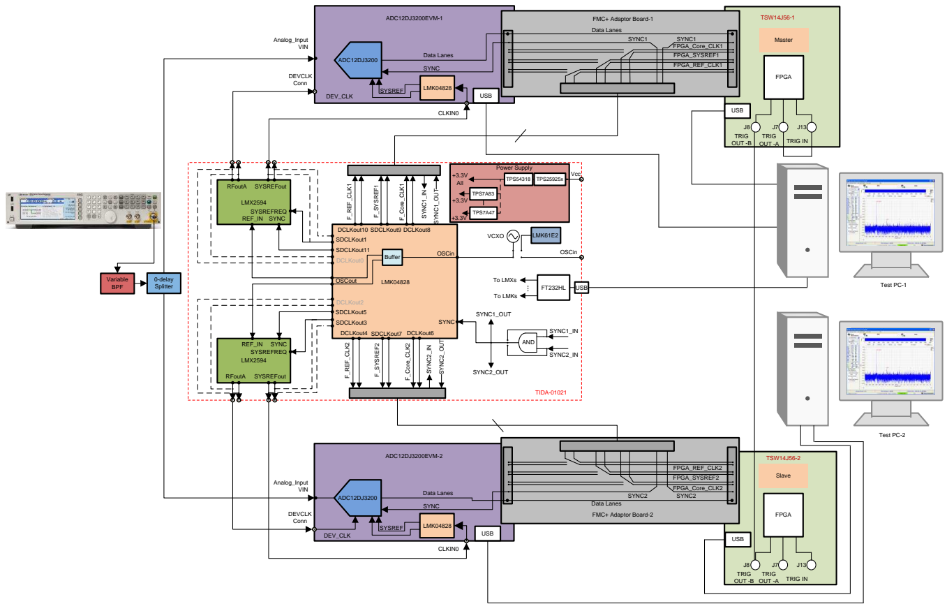
图 9. Test Setup for Channel-to-Channel Skew Measurement
