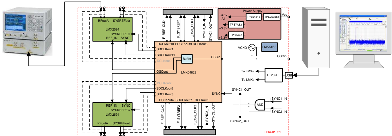
图 6. Test Setup for Phase Noise Measurement
