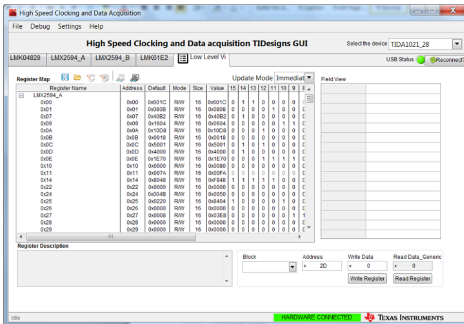
图 4. Clocking Board Programming
