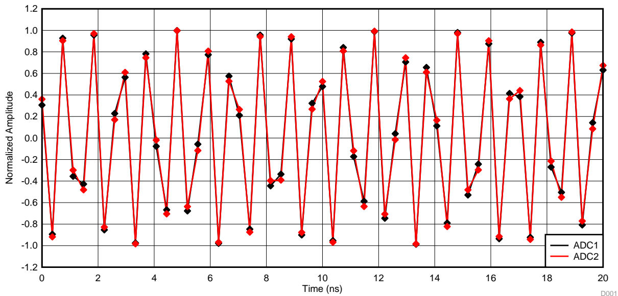
图 17. Sampled Signals at 997-MHz Input
