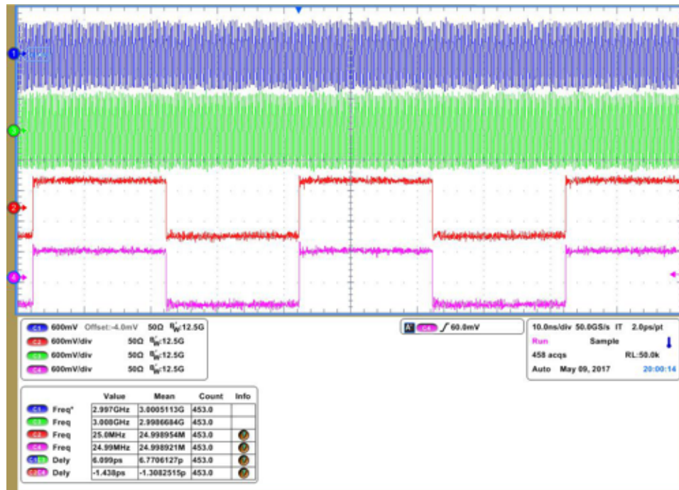
图 13. Multichannel Clock Skew Measurement
