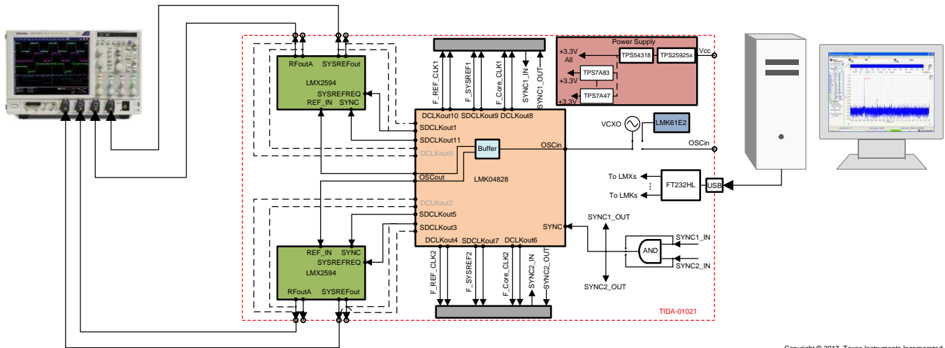
图 7. Test Setup for Multichannel Clock Skew Measurement
