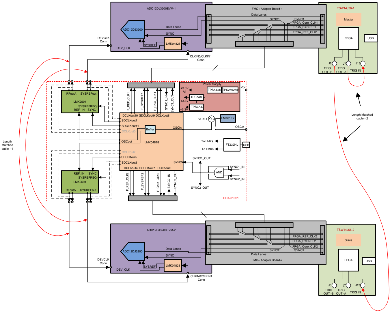
图 1. Block Diagram of Interface Between Clocking Board, ADC12DJ3200 EVM, FMC+ Adaptor Board, and TSW14J56 Board
