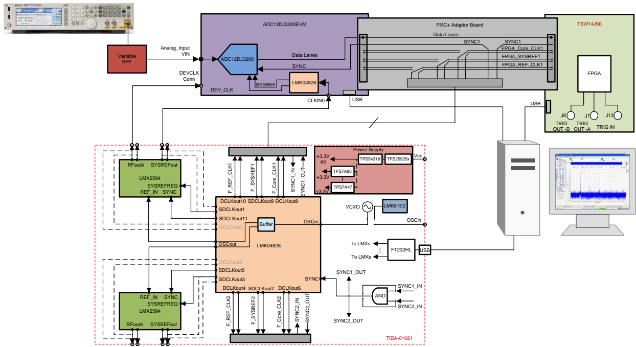
图 8. Test Setup for SNR Measurement
