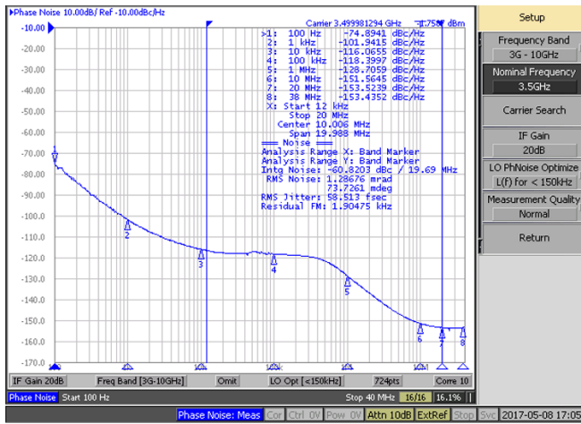
图 10. Phase Noise at 3.5 GHz
