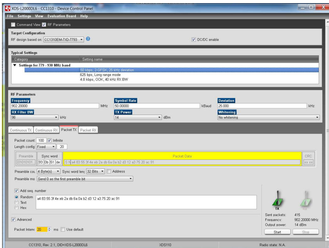
图 30. Non-Continuous Noise at 902.2-MHz Frequency (Channel 0 in FCC Band)
