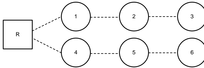
图 39. Multi-Hop Topology With Two Three-Hop Network Branches
