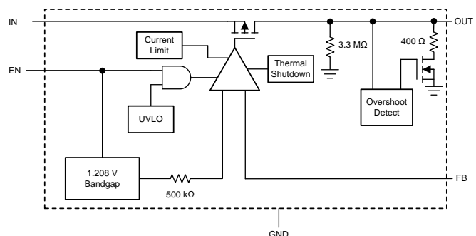
图 8. Functional Block Diagram (Adjustable Voltage Version)
