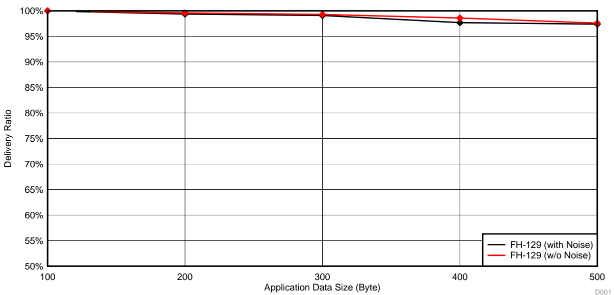
图 31. Delivery Ratio (in %) as a Function of Data Size
