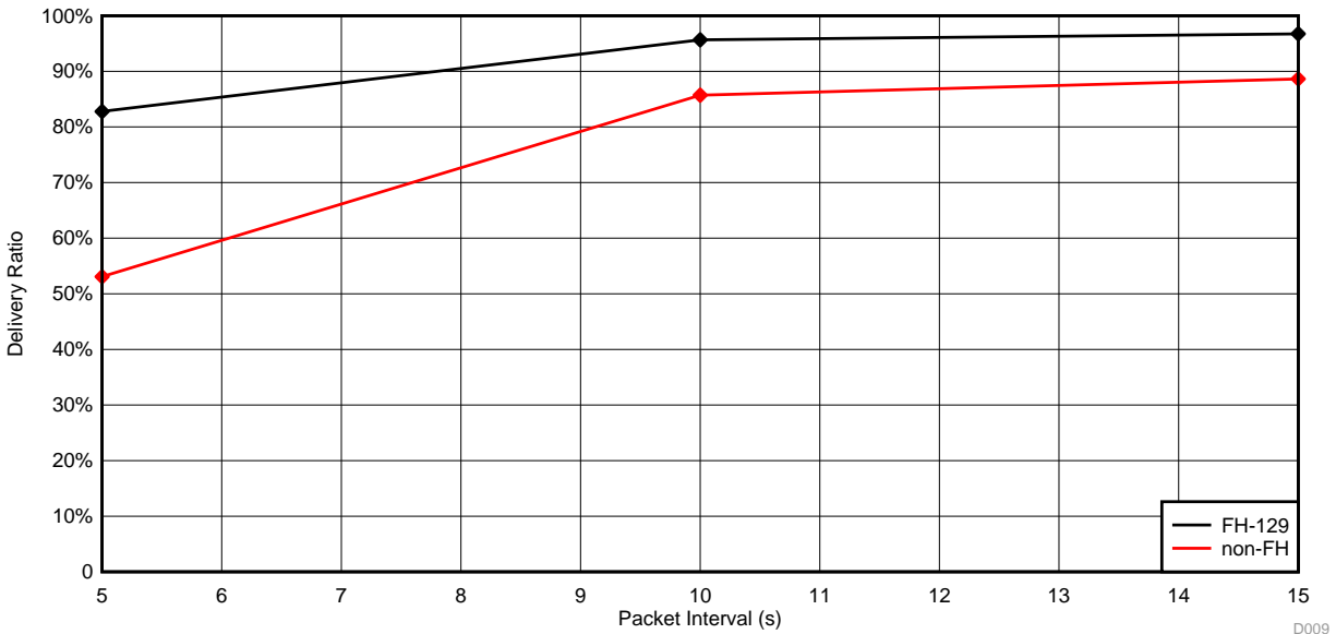
图 40. Delivery Ratio Performance as a Function of Packet Interval
