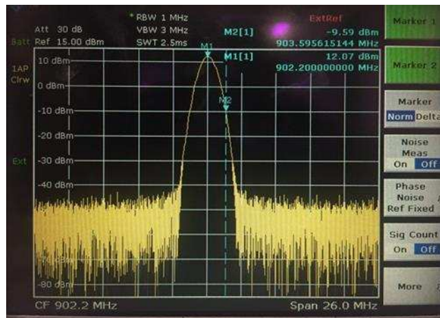
图 29. Spectrum Analyzer Capture for Continuous Noise With TX Power of 14 dBm
