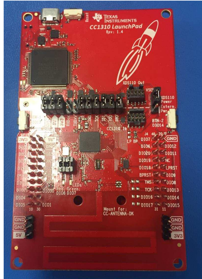
图 11. Hardware Configuration (Top)
