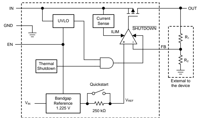
图 6. Functional Block Diagram (Adjustable Version)
