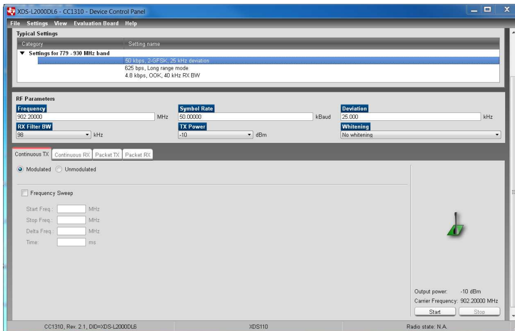
图 28. Continuous Noise at 902.2-MHz Frequency (Channel 0 in FCC Band)
