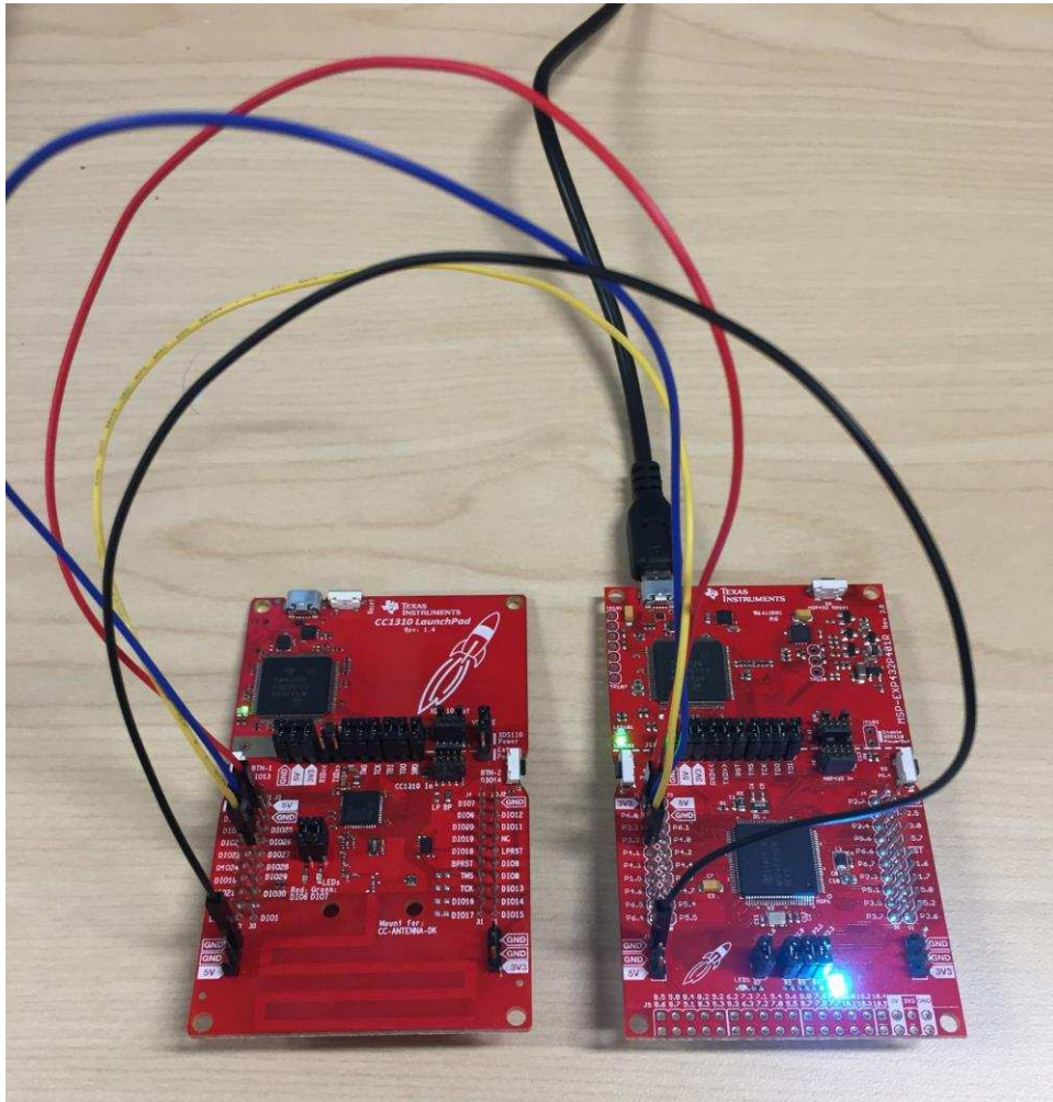
图 12. Wiring-Based Hardware Configuration
