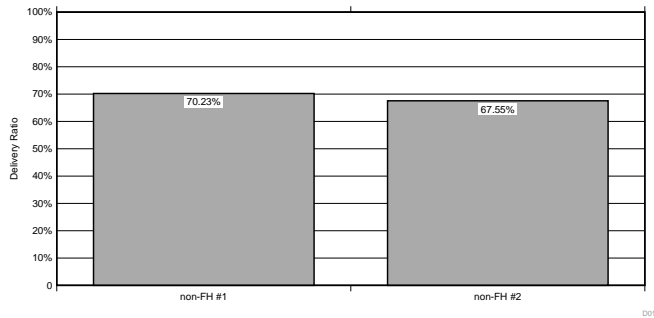
图 43. Delivery Ratio in Non-FH With Non-FH Scenario
