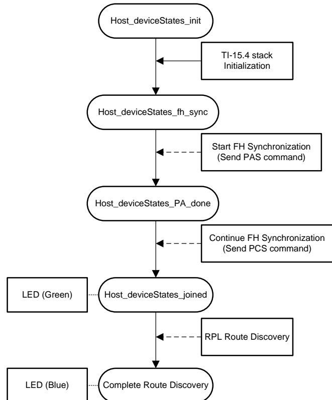
图 18. Software State Machine (End-Node)
