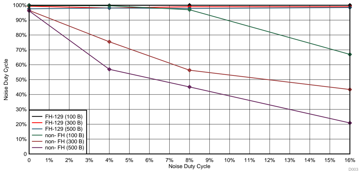
图 33. Delivery Ratio (in %) as a Function of Noise Duty Cycle
