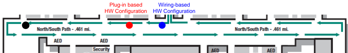
图 13. Communication Range Measurement With Two-Node Setup
