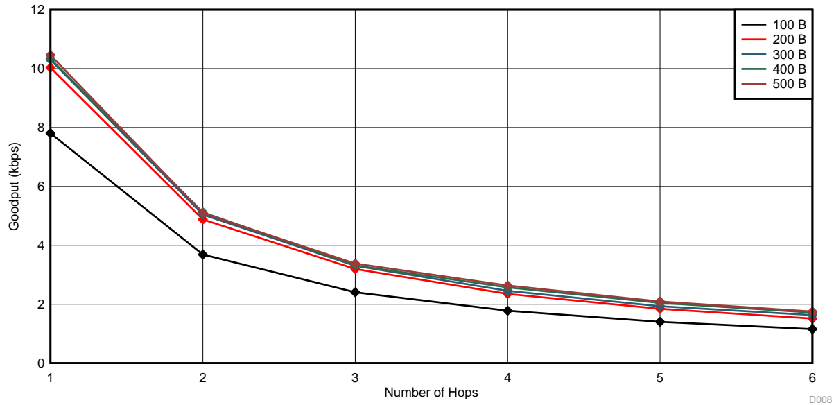
图 38. Goodput Performance (in kbps) as a Function of Number of Hops
