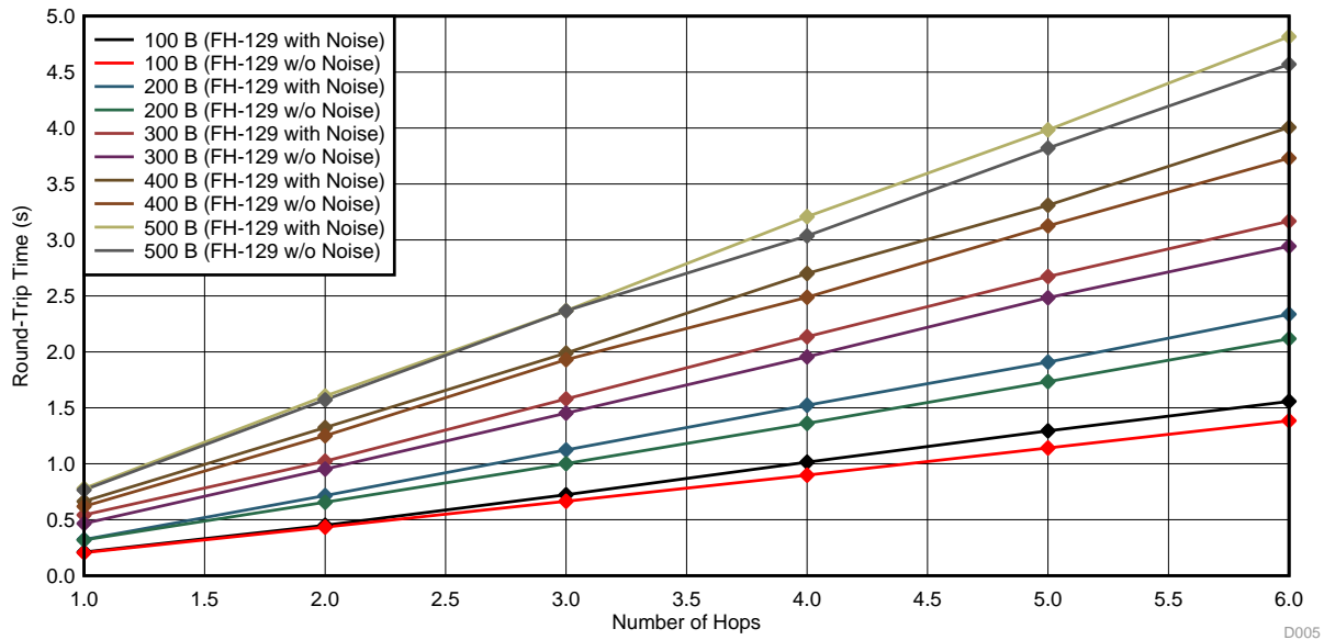
图 35. Round-Trip Time (in Seconds) Over Six-Hop Network
