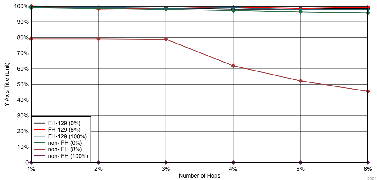
图 34. Delivery Ratio (in %) With Noise Duty Cycle as a Function of Number of Hops
