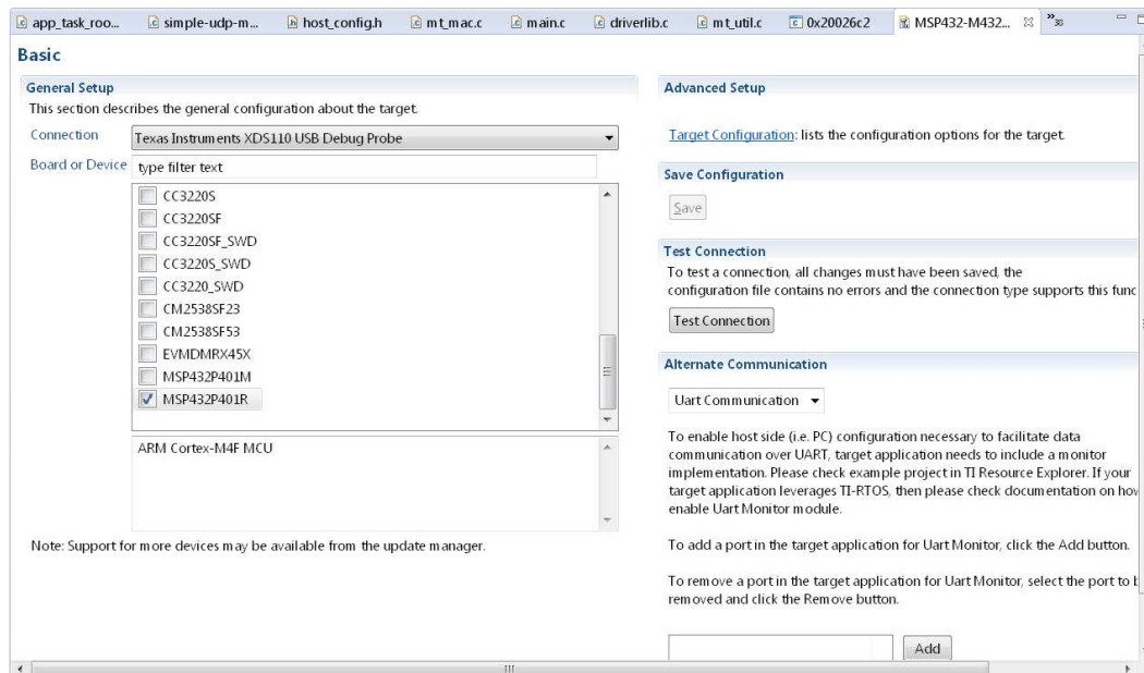
图 23. CCS™ Target Configuration for MSP432™
