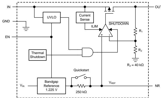
图 5. Functional Block Diagram (Fixed Version)
