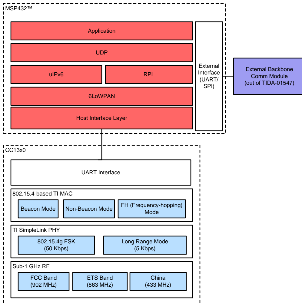
图 1. TIDA-01547 System Architecture
