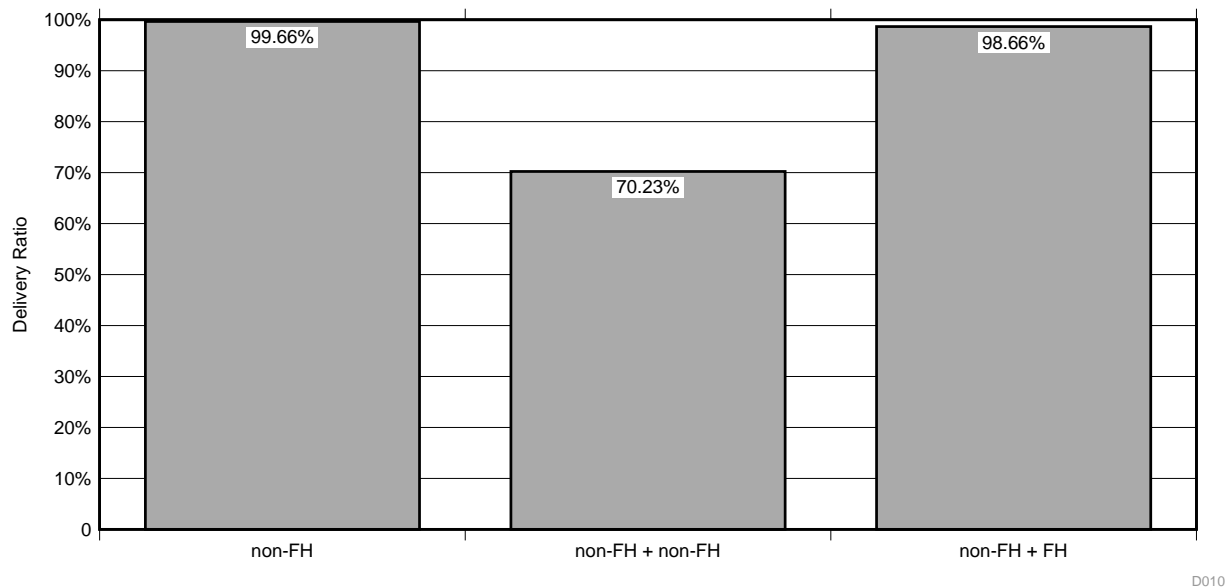
图 42. Delivery Ratio Performance of Non-FH System in Various Coexistence Scenario
