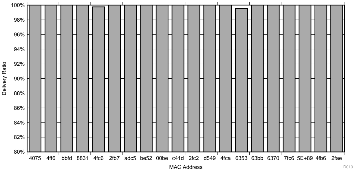
图 46. Delivery Ratio Performance With 100B UDP Polling Example
