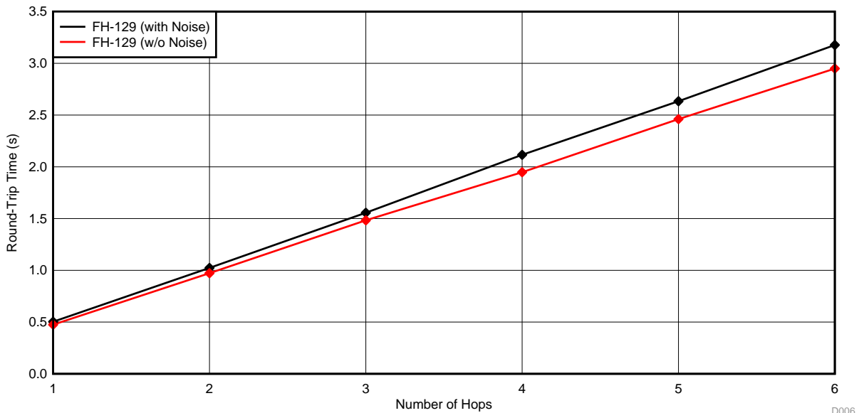
图 36. RTT Performance (in Seconds) as a Function of Number of Hop
