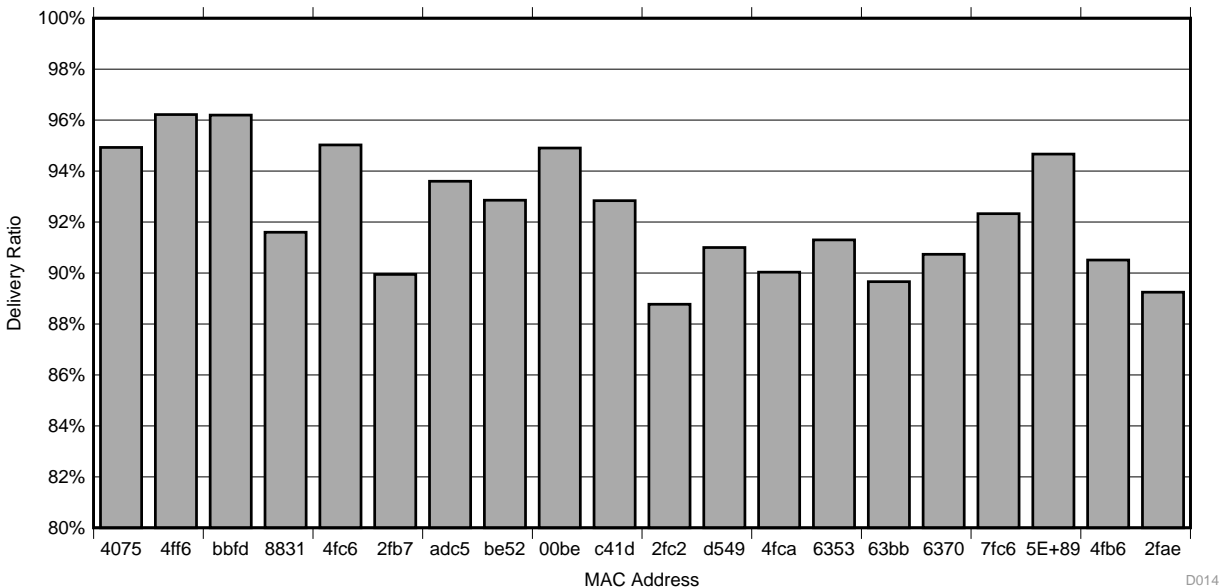
图 47. Delivery Ratio Performance With 500B UDP Polling Example
