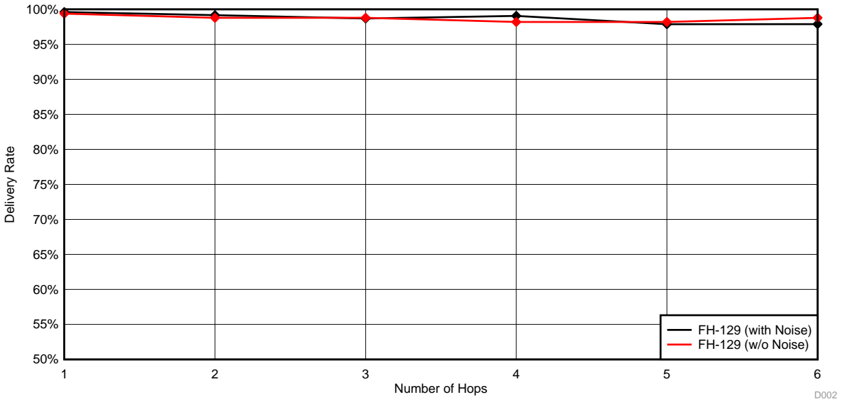
图 32. Delivery Ratio (in %) as a Function of Number of Hops
