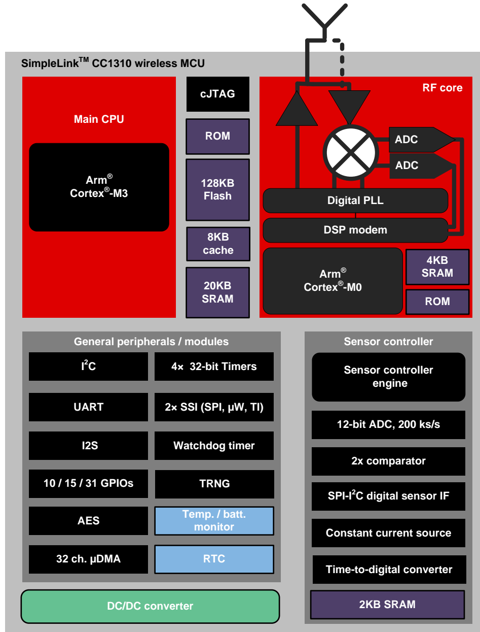
图 4. CC1310 Functional Block Diagram
