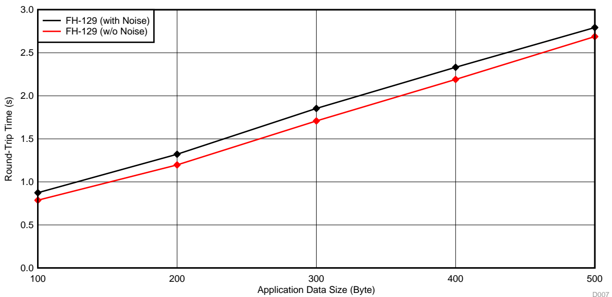
图 37. RTT Performance (in Seconds) as a Function of Data Size
