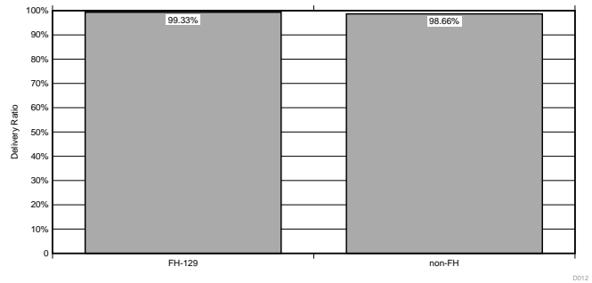
图 44. Delivery Ratio in Non-FH With FH-129 Scenario
