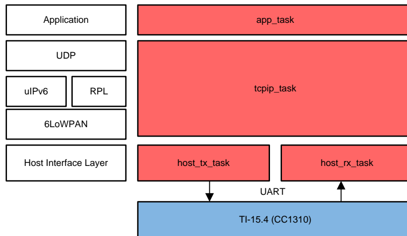
图 19. Software Architecture of TIDA-01547
