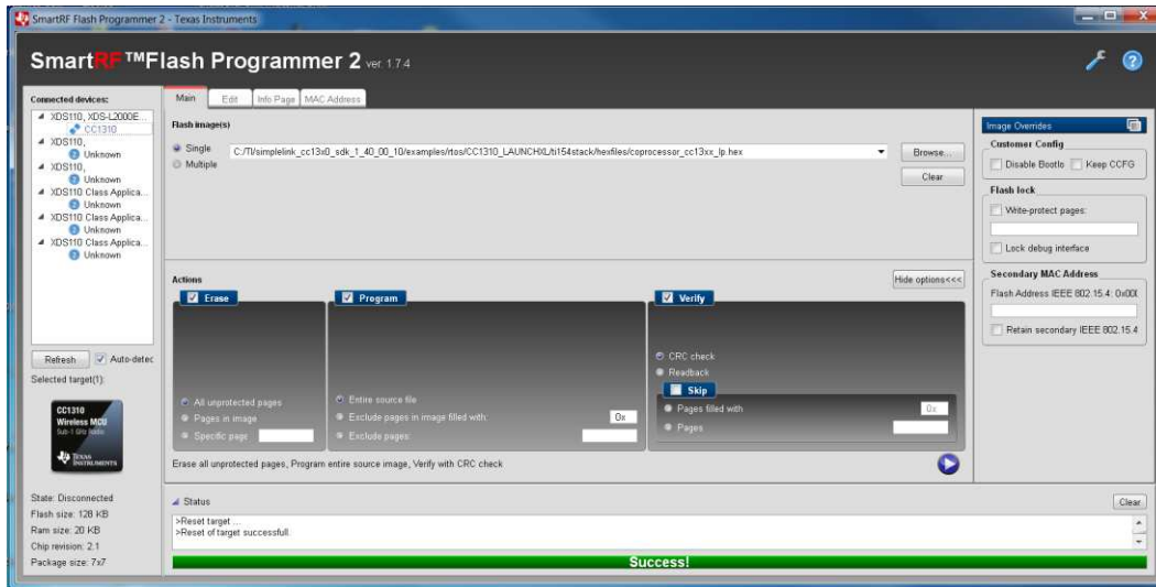
图 25. SmartRF™ Flash Programmer (for TI-15.4 Firmware on CC1310)
