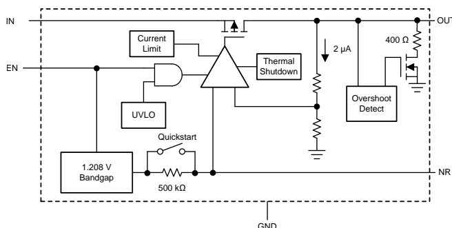
图 7. Functional Block Diagram (Fixed Voltage Version)
