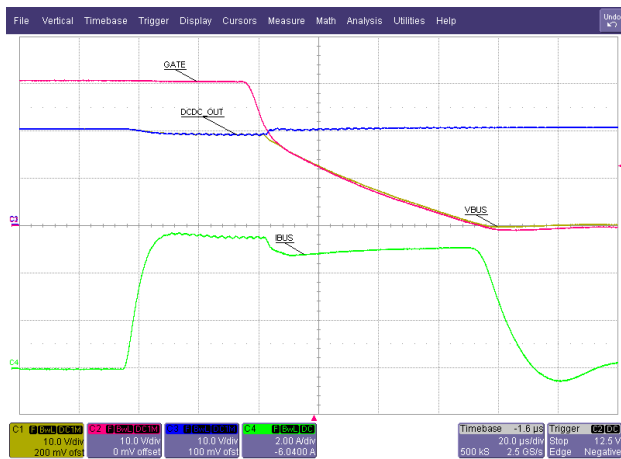
Figure 32. 5.5-A Load Step Triggers OCP (20 V)
