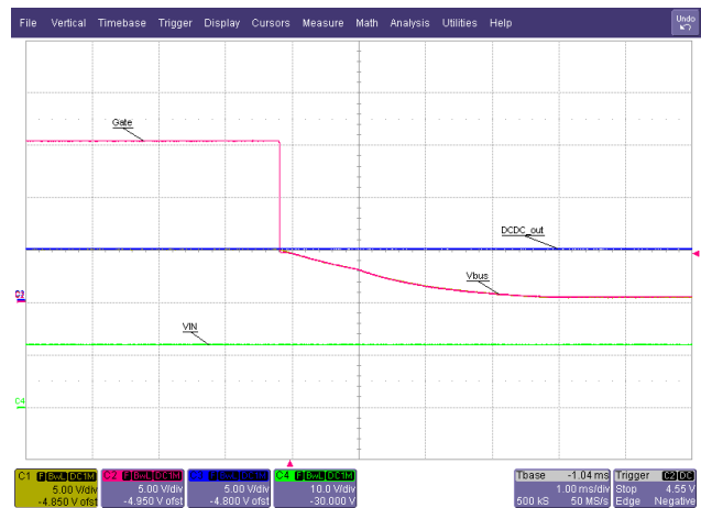
Figure 7. UFP Unplug (5 V)
