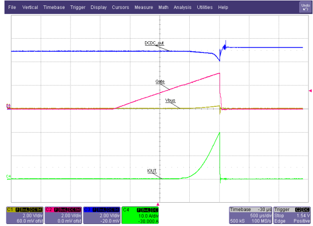
Figure 17. Start Into Short on Output (Extra 1000 µF Between DCDC_out and GND)
