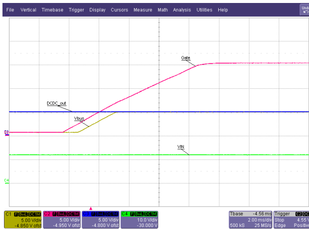
Figure 6. UFP Plug-In (5 V)
