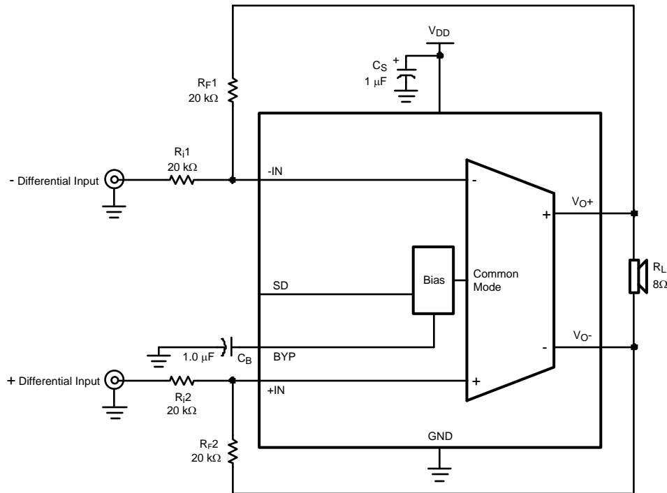
Figure 3. Typical Audio Amplifier Application Circuit
