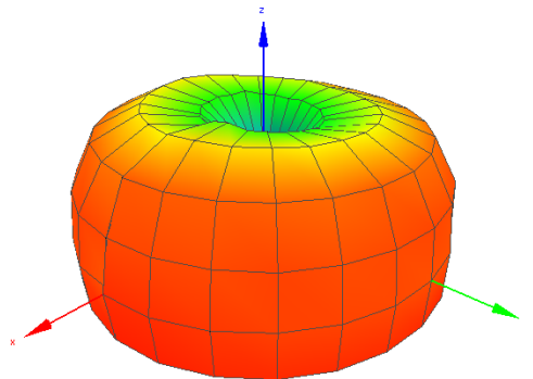
Figure 3. Emission Pattern of a Dipole Antenna
