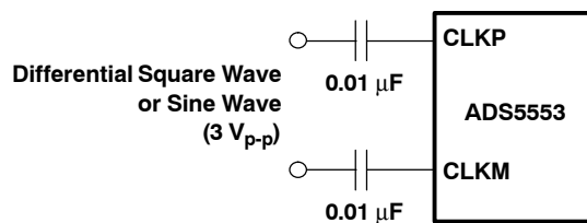
Figure 35. AC-Coupled, Differential Clock Input
